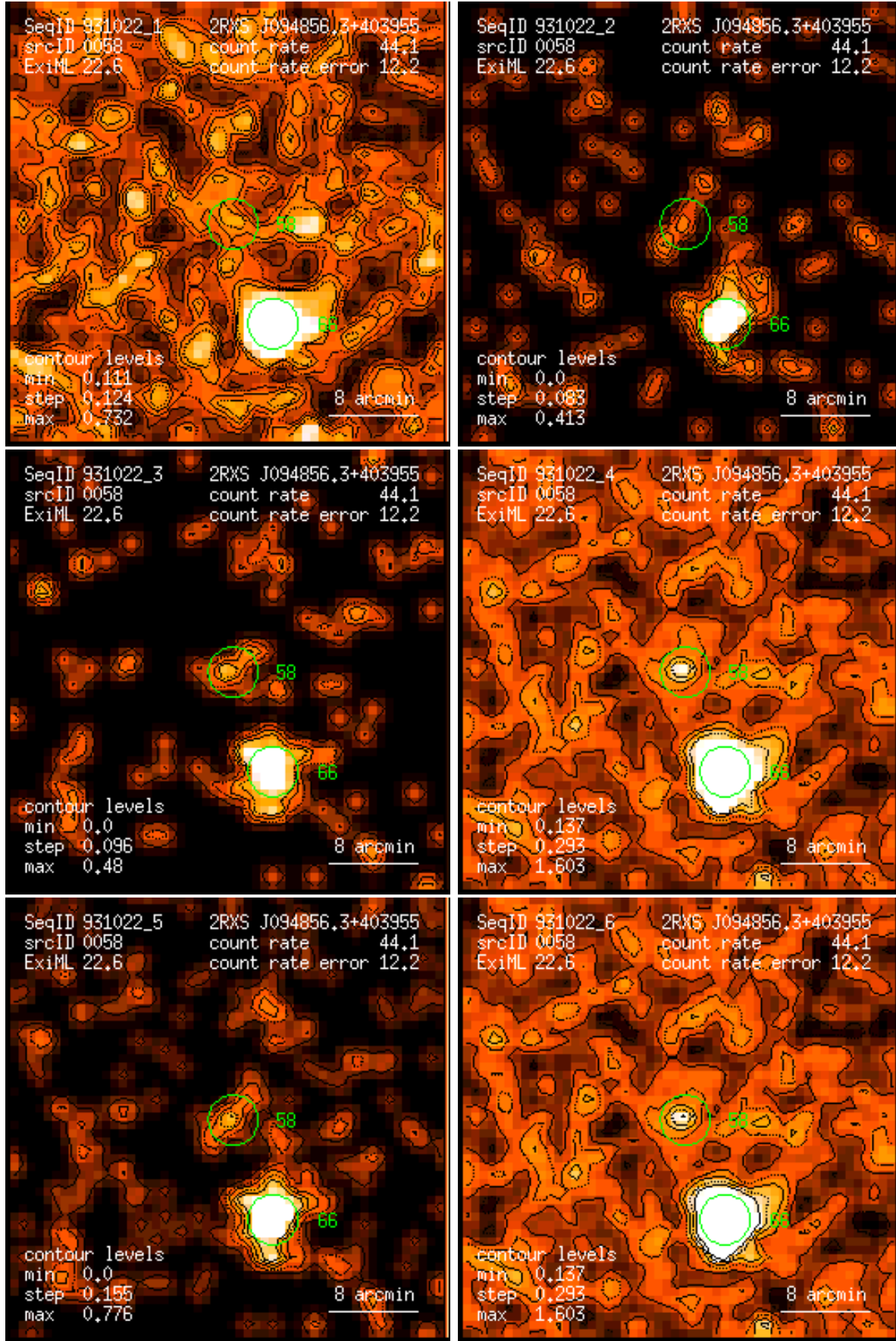
Figure 58: RASS 931022: detection 0058: band rate images, Gaussian filter: (1) PSPC channels 11 – 41, (2) 52 – 90, (3) 91 – 201, (4) 11 – 235, (5) 52 – 201, (6) 11 – 201. Broad band rates in counts/ks. Band rate contour levels in counts/ks/arcmin 2 .
