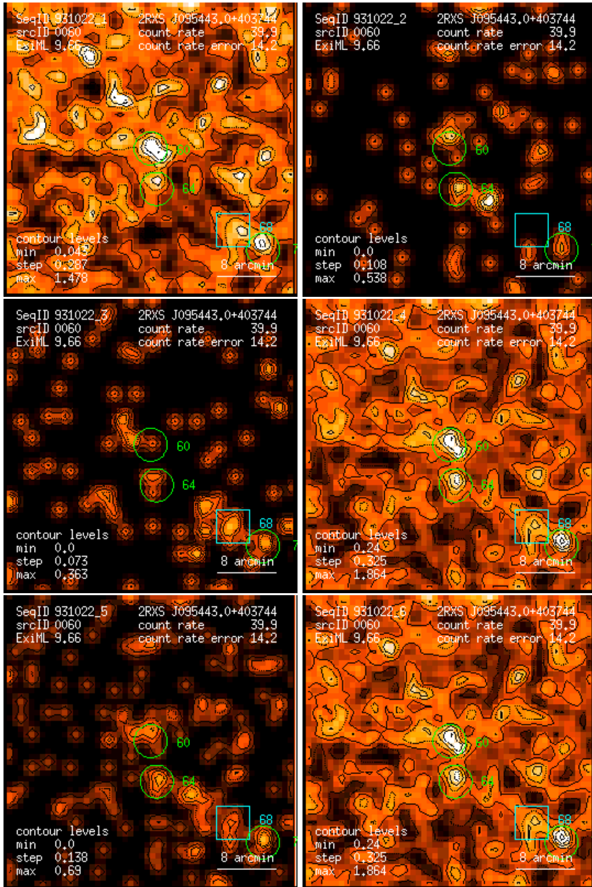
Figure 60: RASS 931022: detection 0060: band rate images, Gaussian filter: (1) PSPC channels 11 – 41, (2) 52 – 90, (3) 91 – 201, (4) 11 – 235, (5) 52 – 201, (6) 11 – 201. Broad band rates in counts/ks. Band rate contour levels in counts/ks/arcmin 2 .
