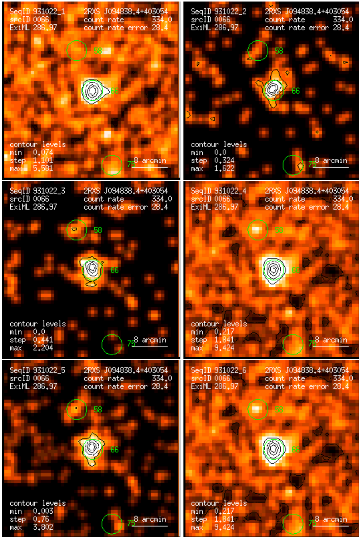
Figure 66: RASS 931022: detection 0066: band rate images, Gaussian filter: (1) PSPC channels 11 – 41, (2) 52 – 90, (3) 91 – 201, (4) 11 – 235, (5) 52 – 201, (6) 11 – 201. Broad band rates in counts/ks. Band rate contour levels in counts/ks/arcmin 2 .
