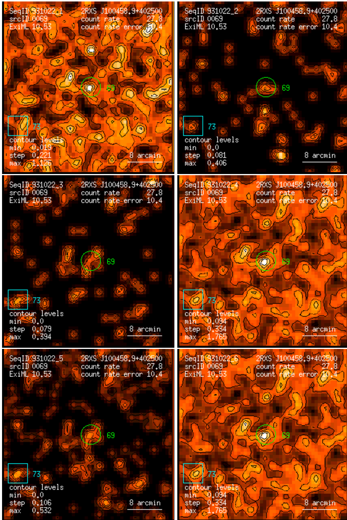
Figure 69: RASS 931022: detection 0069: band rate images, Gaussian filter: (1) PSPC channels 11 – 41, (2) 52 – 90, (3) 91 – 201, (4) 11 – 235, (5) 52 – 201, (6) 11 – 201. Broad band rates in counts/ks. Band rate contour levels in counts/ks/arcmin 2 .
