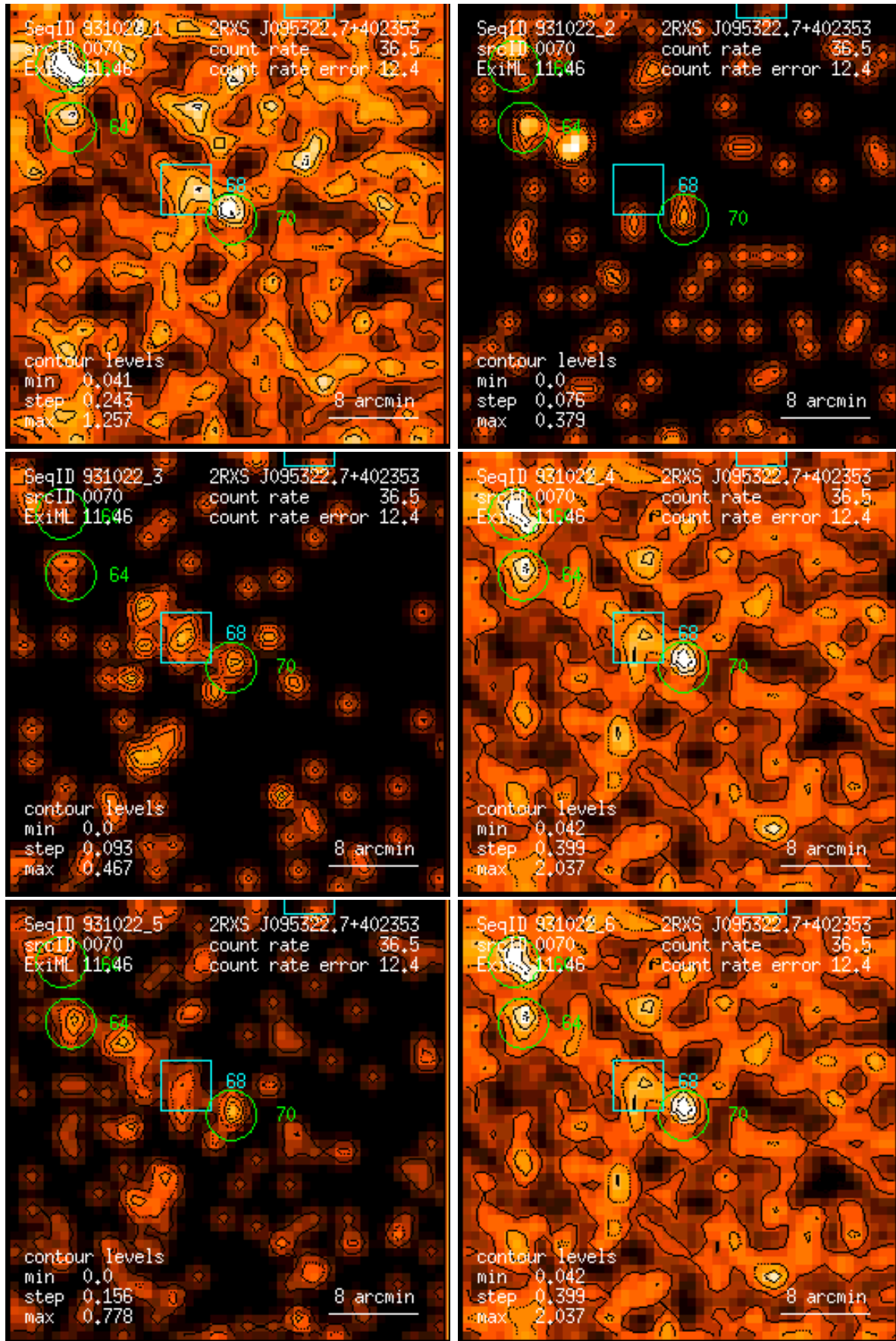
Figure 70: RASS 931022: detection 0070: band rate images, Gaussian filter: (1) PSPC channels 11 – 41, (2) 52 – 90, (3) 91 – 201, (4) 11 – 235, (5) 52 – 201, (6) 11 – 201. Broad band rates in counts/ks. Band rate contour levels in counts/ks/arcmin 2 .
