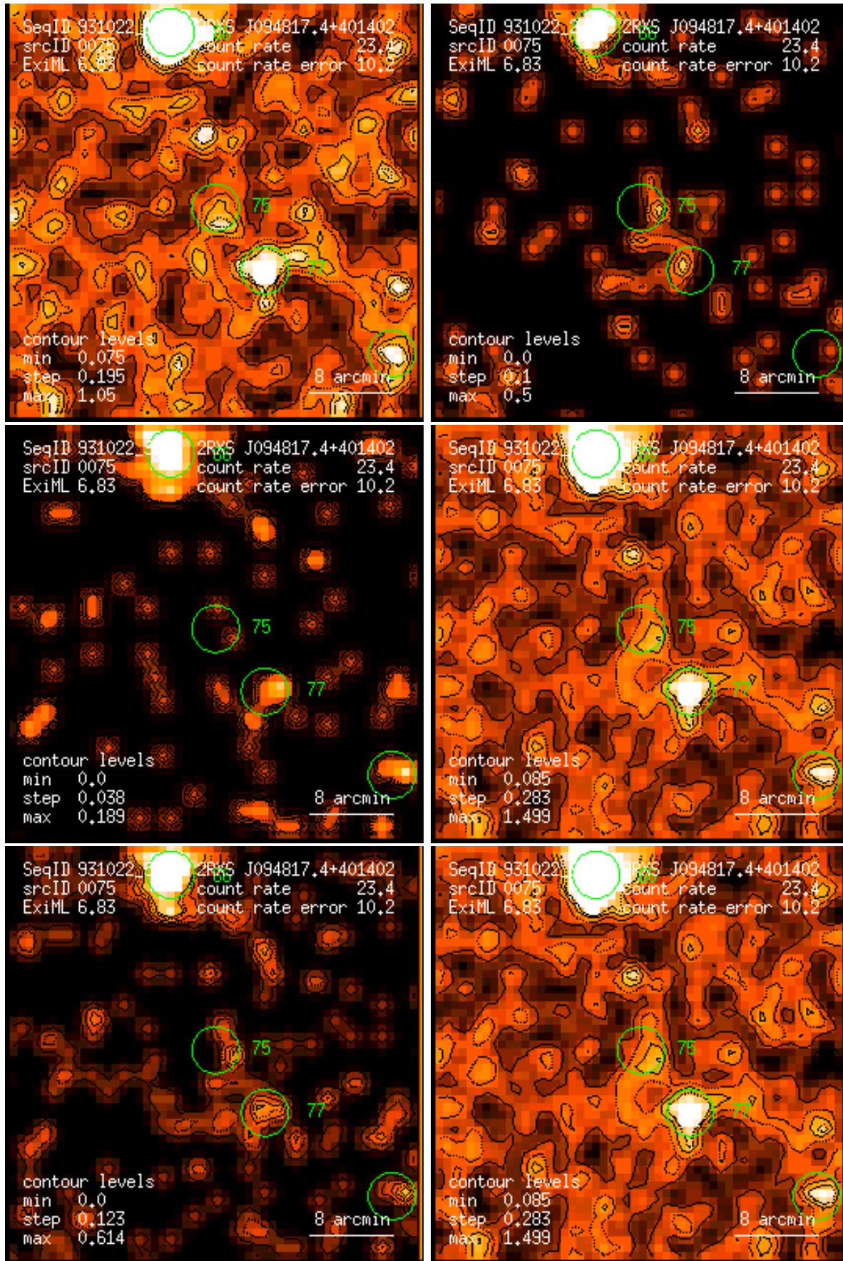
Figure 75: RASS 931022: detection 0075: band rate images, Gaussian filter: (1) PSPC channels 11 – 41, (2) 52 – 90, (3) 91 – 201, (4) 11 – 235, (5) 52 – 201, (6) 11 – 201. Broad band rates in counts/ks. Band rate contour levels in counts/ks/arcmin 2 .
