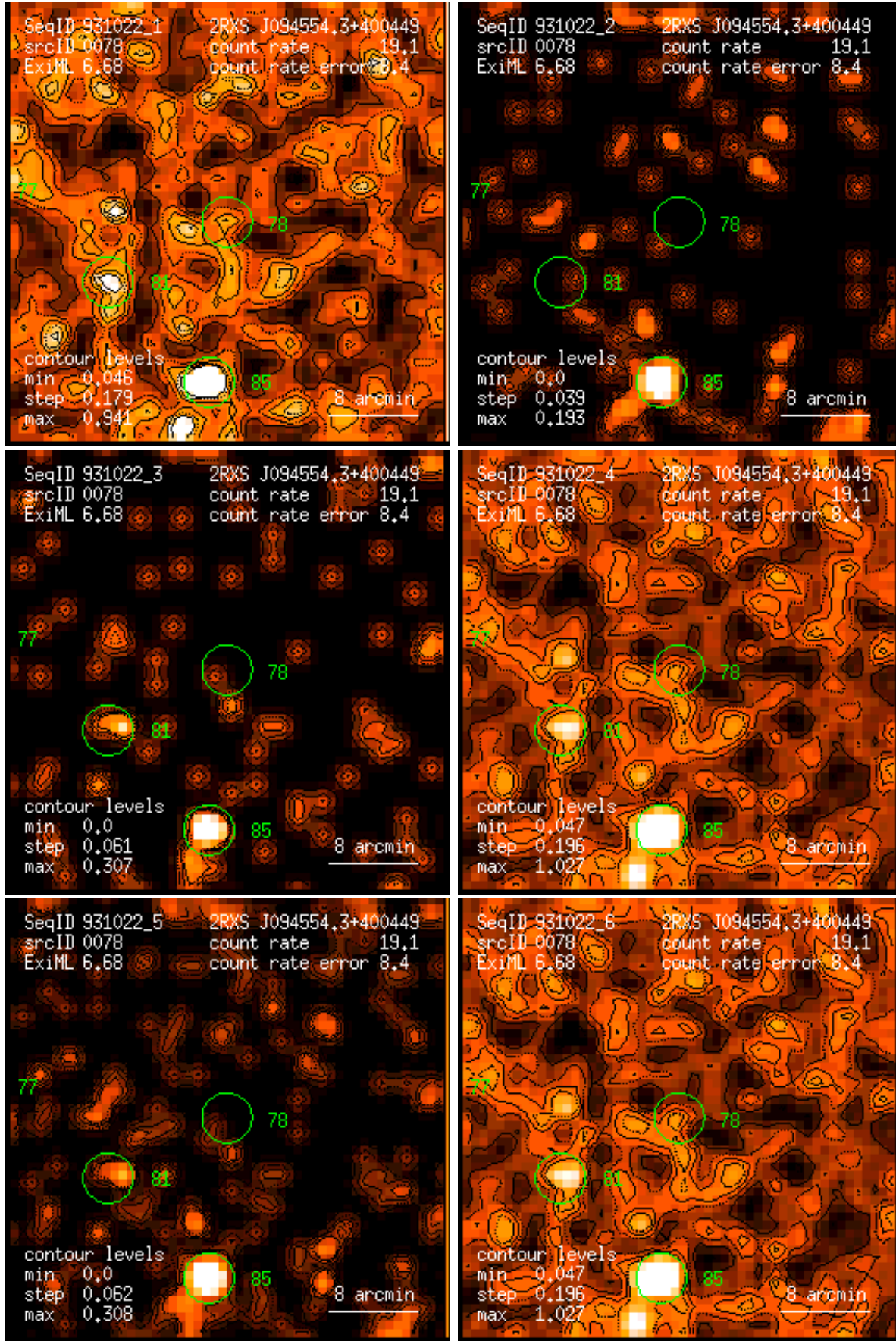
Figure 78: RASS 931022: detection 0078: band rate images, Gaussian filter: (1) PSPC channels 11 – 41, (2) 52 – 90, (3) 91 – 201, (4) 11 – 235, (5) 52 – 201, (6) 11 – 201. Broad band rates in counts/ks. Band rate contour levels in counts/ks/arcmin 2 .
