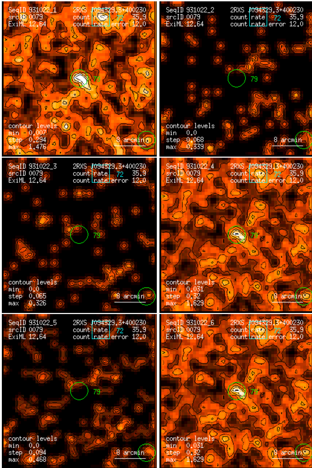
Figure 79: RASS 931022: detection 0079: band rate images, Gaussian filter: (1) PSPC channels 11 – 41, (2) 52 – 90, (3) 91 – 201, (4) 11 – 235, (5) 52 – 201, (6) 11 – 201. Broad band rates in counts/ks. Band rate contour levels in counts/ks/arcmin 2 .
