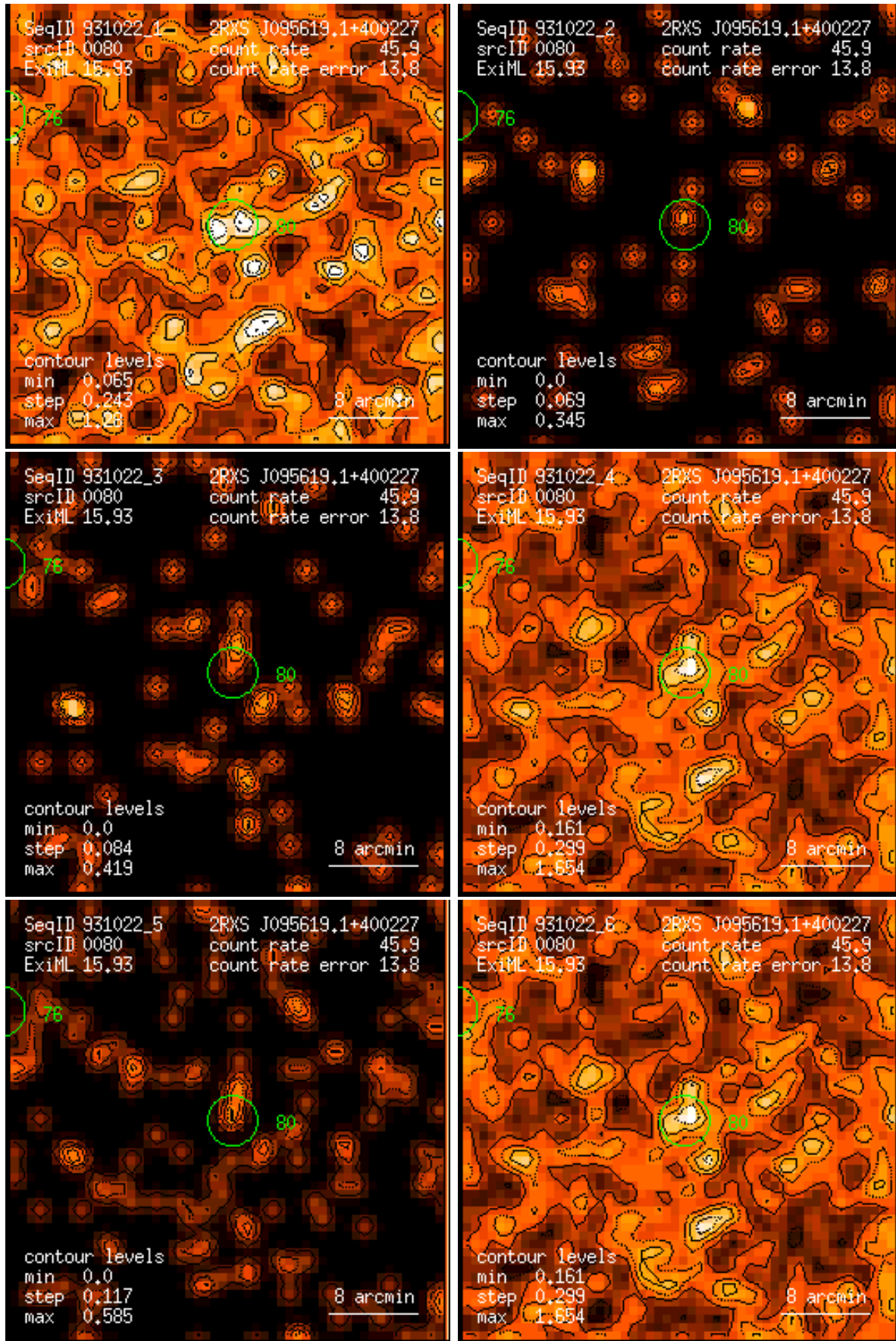
Figure 80: RASS 931022: detection 0080: band rate images, Gaussian filter: (1) PSPC channels 11 – 41, (2) 52 – 90, (3) 91 – 201, (4) 11 – 235, (5) 52 – 201, (6) 11 – 201. Broad band rates in counts/ks. Band rate contour levels in counts/ks/arcmin 2 .
