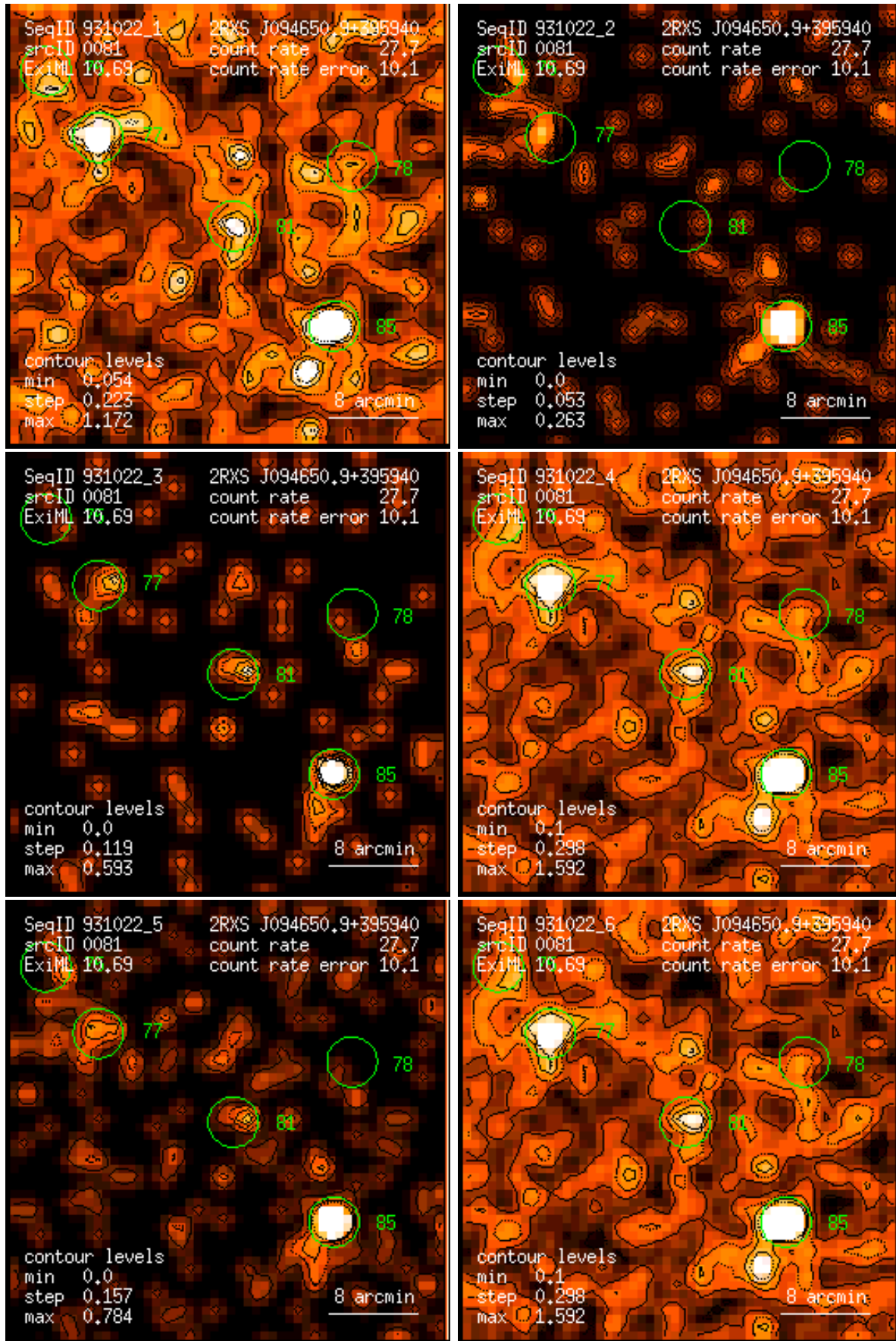
Figure 81: RASS 931022: detection 0081: band rate images, Gaussian filter: (1) PSPC channels 11 – 41, (2) 52 – 90, (3) 91 – 201, (4) 11 – 235, (5) 52 – 201, (6) 11 – 201. Broad band rates in counts/ks. Band rate contour levels in counts/ks/arcmin 2 .
