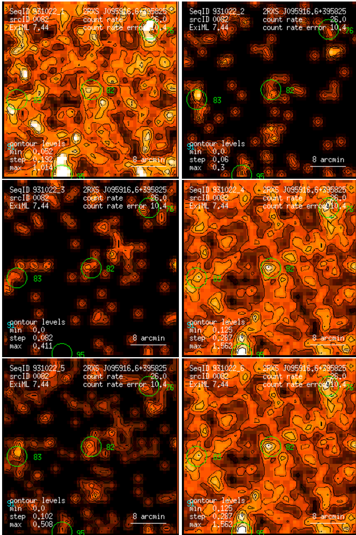
Figure 82: RASS 931022: detection 0082: band rate images, Gaussian filter: (1) PSPC channels 11 – 41, (2) 52 – 90, (3) 91 – 201, (4) 11 – 235, (5) 52 – 201, (6) 11 – 201. Broad band rates in counts/ks. Band rate contour levels in counts/ks/arcmin 2 .
