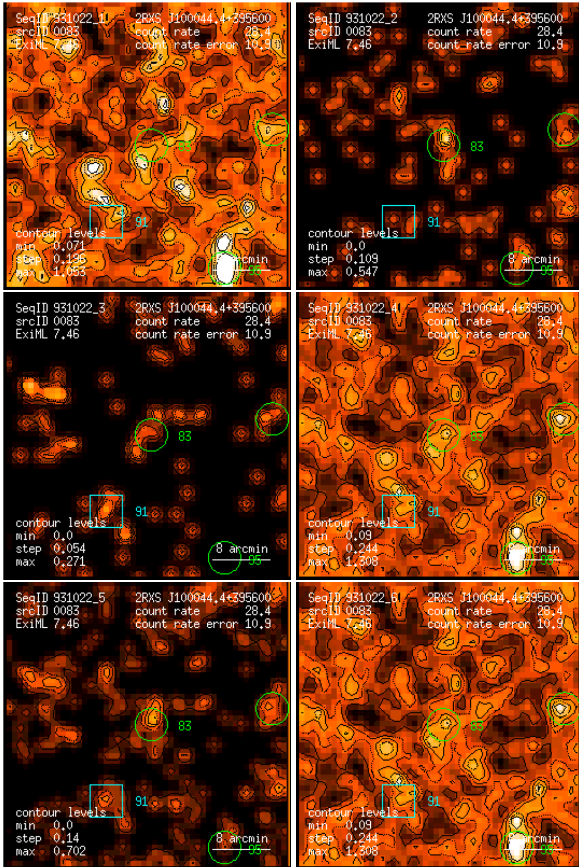
Figure 83: RASS 931022: detection 0083: band rate images, Gaussian filter: (1) PSPC channels 11 – 41, (2) 52 – 90, (3) 91 – 201, (4) 11 – 235, (5) 52 – 201, (6) 11 – 201. Broad band rates in counts/ks. Band rate contour levels in counts/ks/arcmin 2 .
