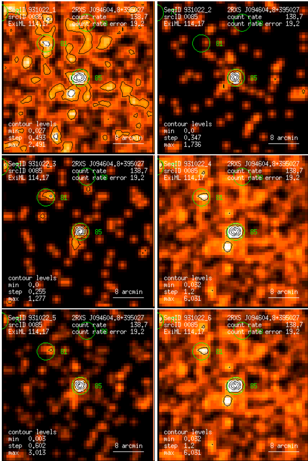
Figure 85: RASS 931022: detection 0085: band rate images, Gaussian filter: (1) PSPC channels 11 – 41, (2) 52 – 90, (3) 91 – 201, (4) 11 – 235, (5) 52 – 201, (6) 11 – 201. Broad band rates in counts/ks. Band rate contour levels in counts/ks/arcmin 2 .
