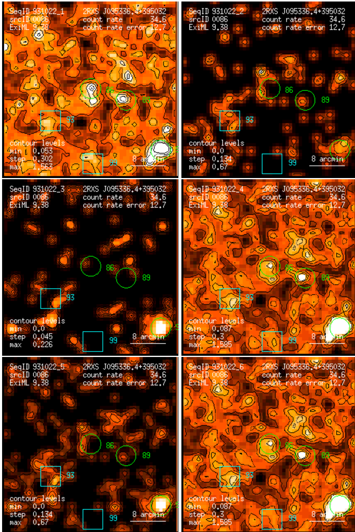
Figure 86: RASS 931022: detection 0086: band rate images, Gaussian filter: (1) PSPC channels 11 – 41, (2) 52 – 90, (3) 91 – 201, (4) 11 – 235, (5) 52 – 201, (6) 11 – 201. Broad band rates in counts/ks. Band rate contour levels in counts/ks/arcmin 2 .
