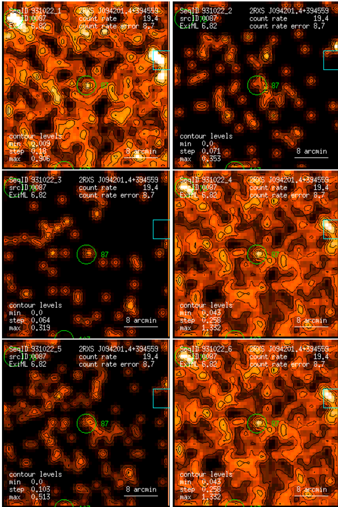
Figure 87: RASS 931022: detection 0087: band rate images, Gaussian filter: (1) PSPC channels 11 – 41, (2) 52 – 90, (3) 91 – 201, (4) 11 – 235, (5) 52 – 201, (6) 11 – 201. Broad band rates in counts/ks. Band rate contour levels in counts/ks/arcmin 2 .
