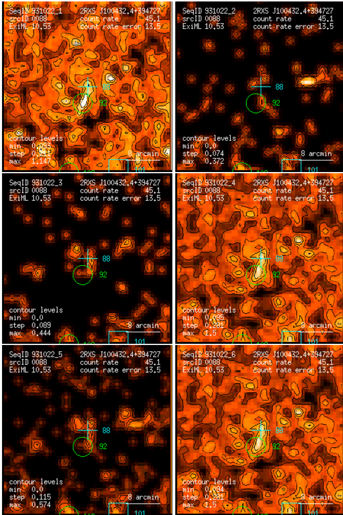
Figure 88: RASS 931022: detection 0088: band rate images, Gaussian filter: (1) PSPC channels 11 – 41, (2) 52 – 90, (3) 91 – 201, (4) 11 – 235, (5) 52 – 201, (6) 11 – 201. Broad band rates in counts/ks. Band rate contour levels in counts/ks/arcmin 2 .
