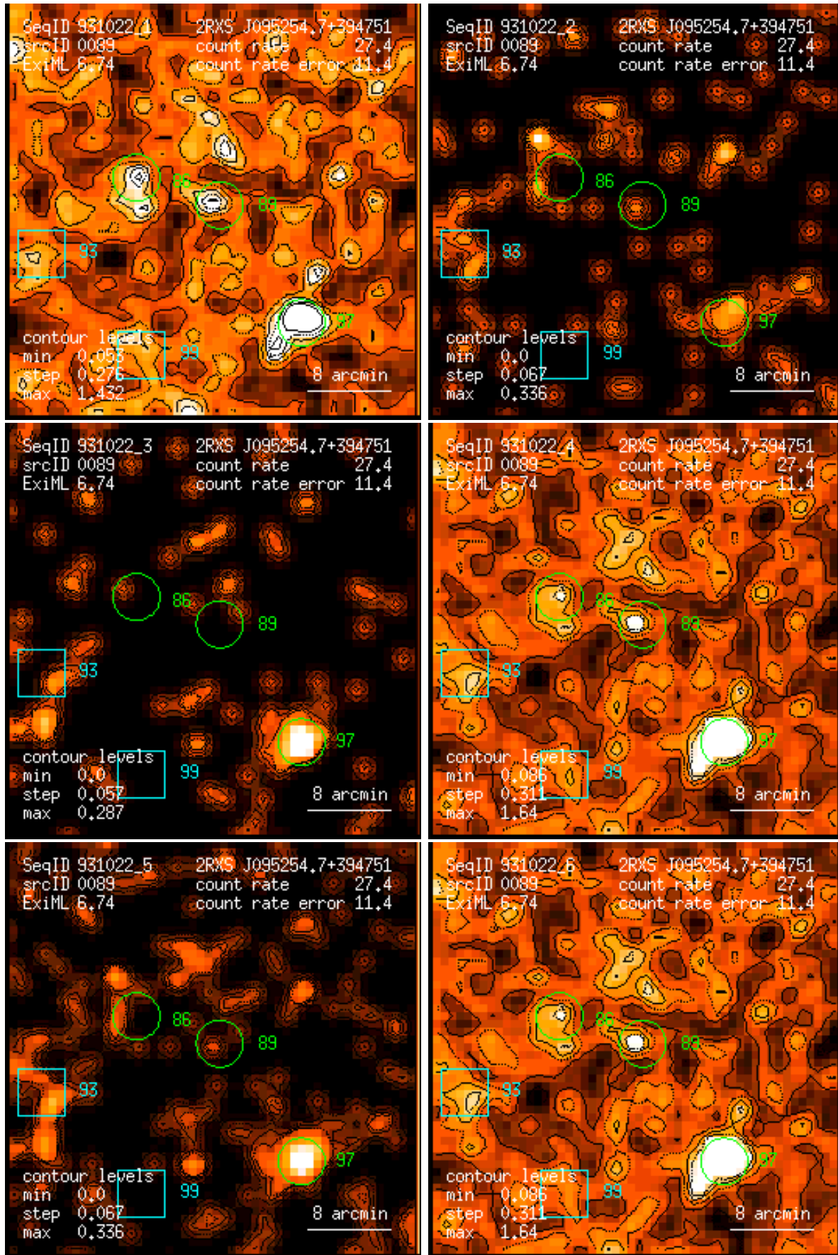
Figure 89: RASS 931022: detection 0089: band rate images, Gaussian filter: (1) PSPC channels 11 – 41, (2) 52 – 90, (3) 91 – 201, (4) 11 – 235, (5) 52 – 201, (6) 11 – 201. Broad band rates in counts/ks. Band rate contour levels in counts/ks/arcmin 2 .
