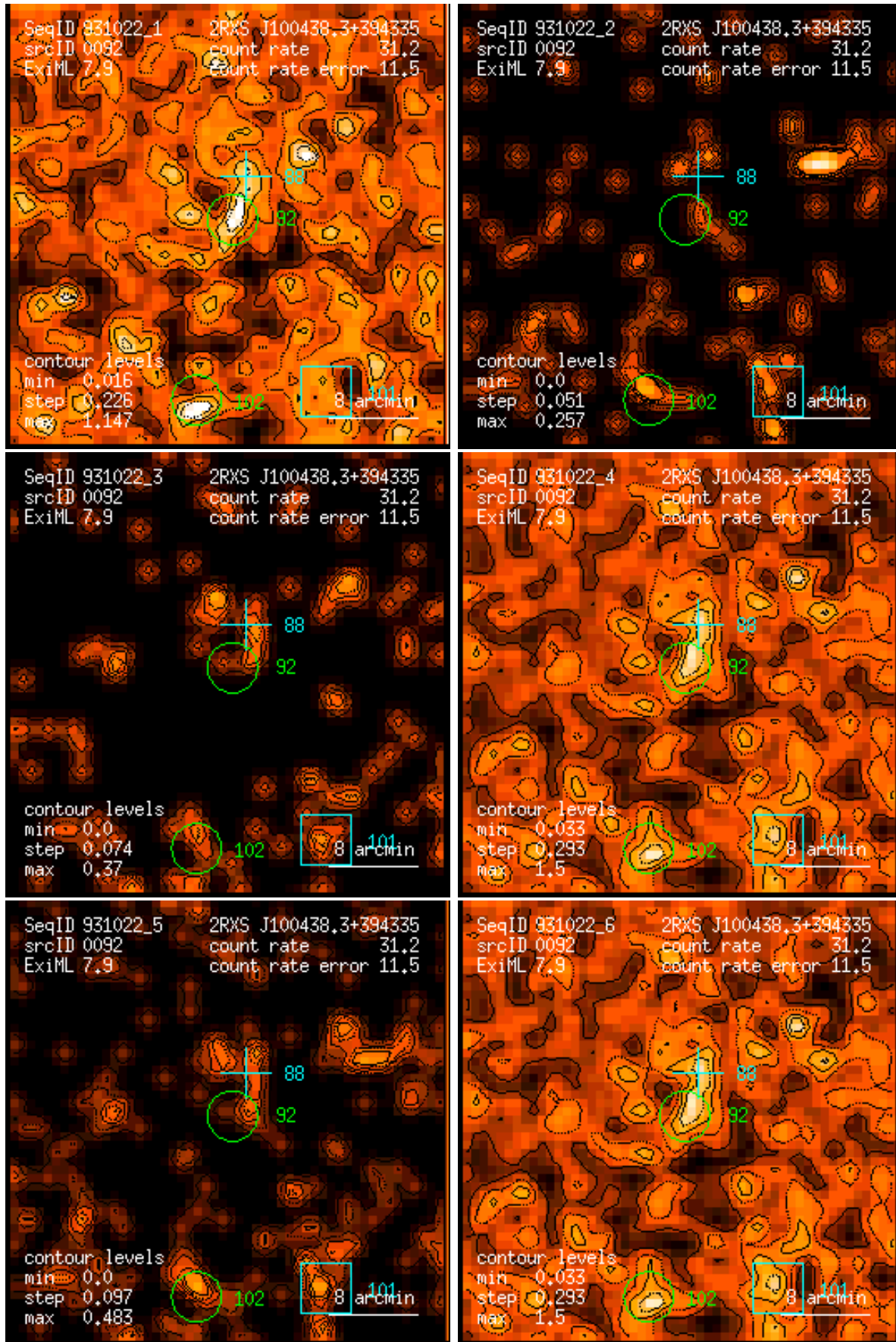
Figure 92: RASS 931022: detection 0092: band rate images, Gaussian filter: (1) PSPC channels 11 – 41, (2) 52 – 90, (3) 91 – 201, (4) 11 – 235, (5) 52 – 201, (6) 11 – 201. Broad band rates in counts/ks. Band rate contour levels in counts/ks/arcmin 2 .
