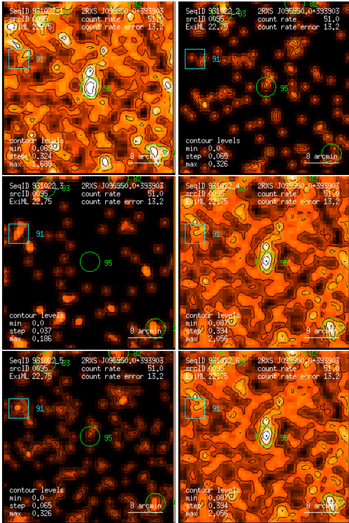
Figure 95: RASS 931022: detection 0095: band rate images, Gaussian filter: (1) PSPC channels 11 – 41, (2) 52 – 90, (3) 91 – 201, (4) 11 – 235, (5) 52 – 201, (6) 11 – 201. Broad band rates in counts/ks. Band rate contour levels in counts/ks/arcmin 2 .
