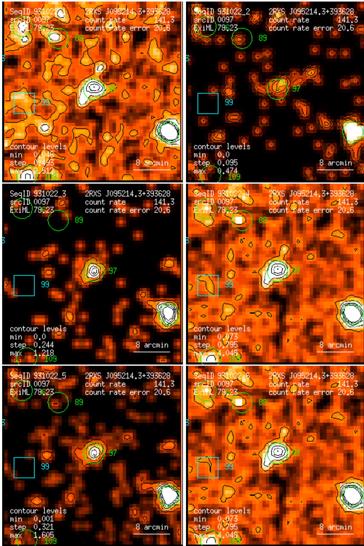
Figure 97: RASS 931022: detection 0097: band rate images, Gaussian filter: (1) PSPC channels 11 – 41, (2) 52 – 90, (3) 91 – 201, (4) 11 – 235, (5) 52 – 201, (6) 11 – 201. Broad band rates in counts/ks. Band rate contour levels in counts/ks/arcmin 2 .
