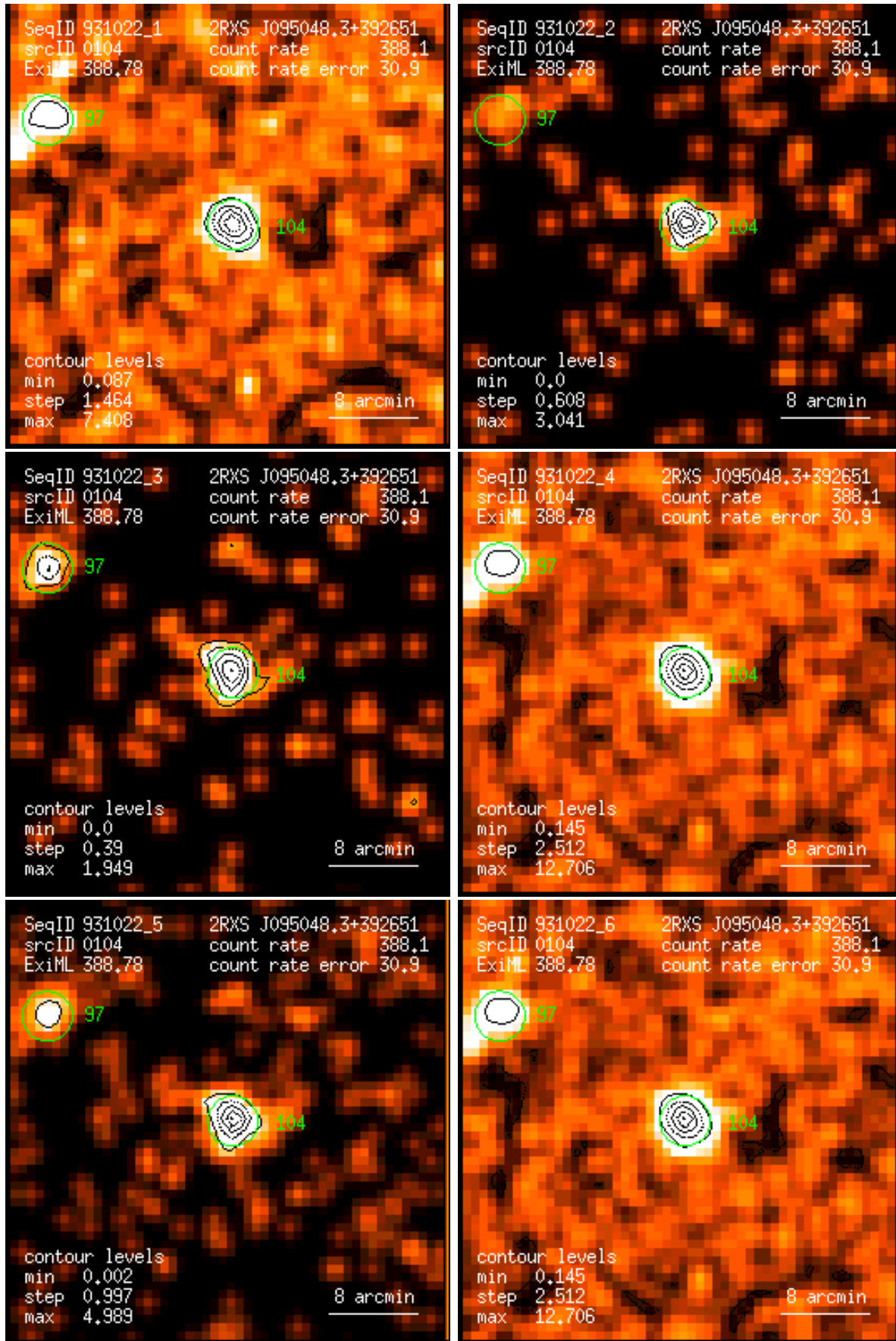
Figure 104: RASS 931022: detection 0104: band rate images, Gaussian filter: (1) PSPC channels 11 – 41, (2) 52 – 90, (3) 91 – 201, (4) 11 – 235, (5) 52 – 201, (6) 11 – 201. Broad band rates in counts/ks. Band rate contour levels in counts/ks/arcmin 2 .
