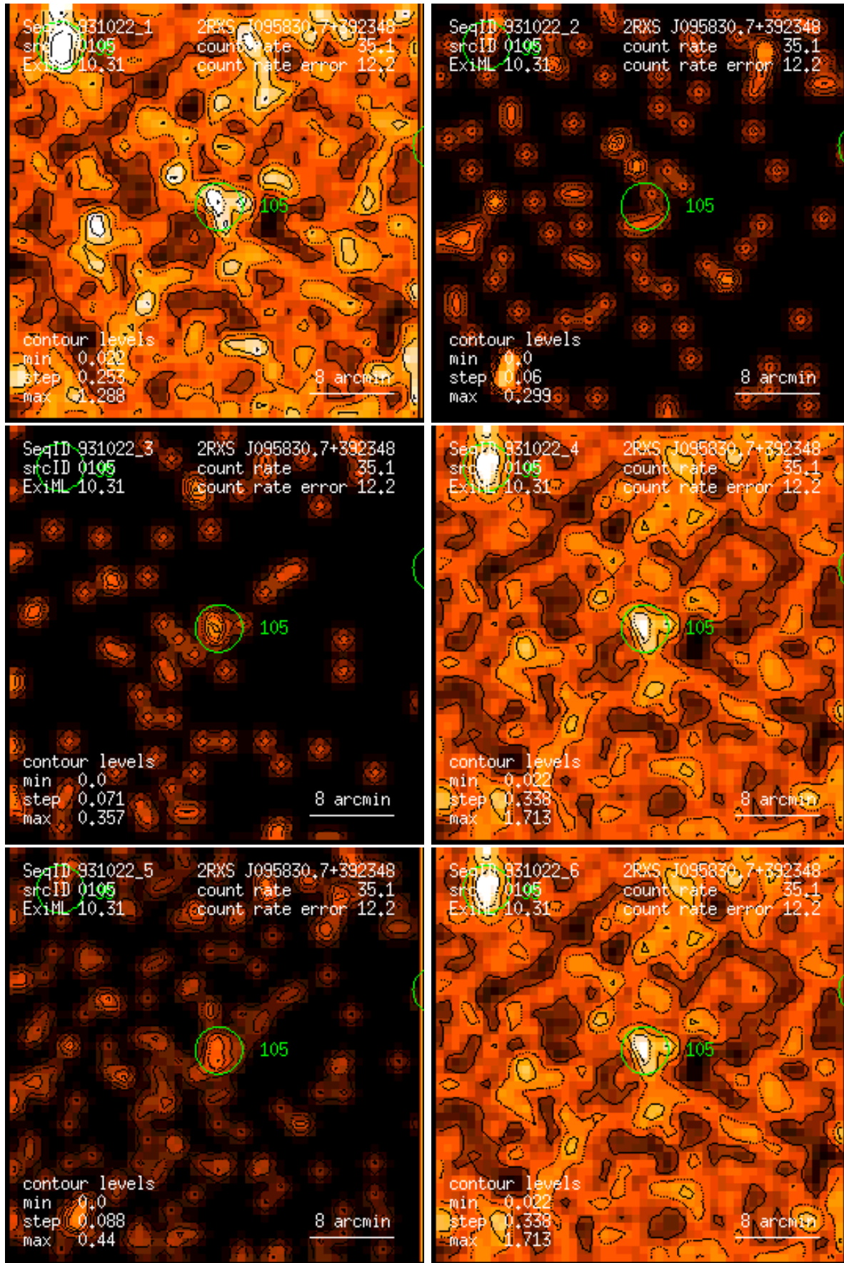
Figure 105: RASS 931022: detection 0105: band rate images, Gaussian filter: (1) PSPC channels 11 – 41, (2) 52 – 90, (3) 91 – 201, (4) 11 – 235, (5) 52 – 201, (6) 11 – 201. Broad band rates in counts/ks. Band rate contour levels in counts/ks/arcmin 2 .
