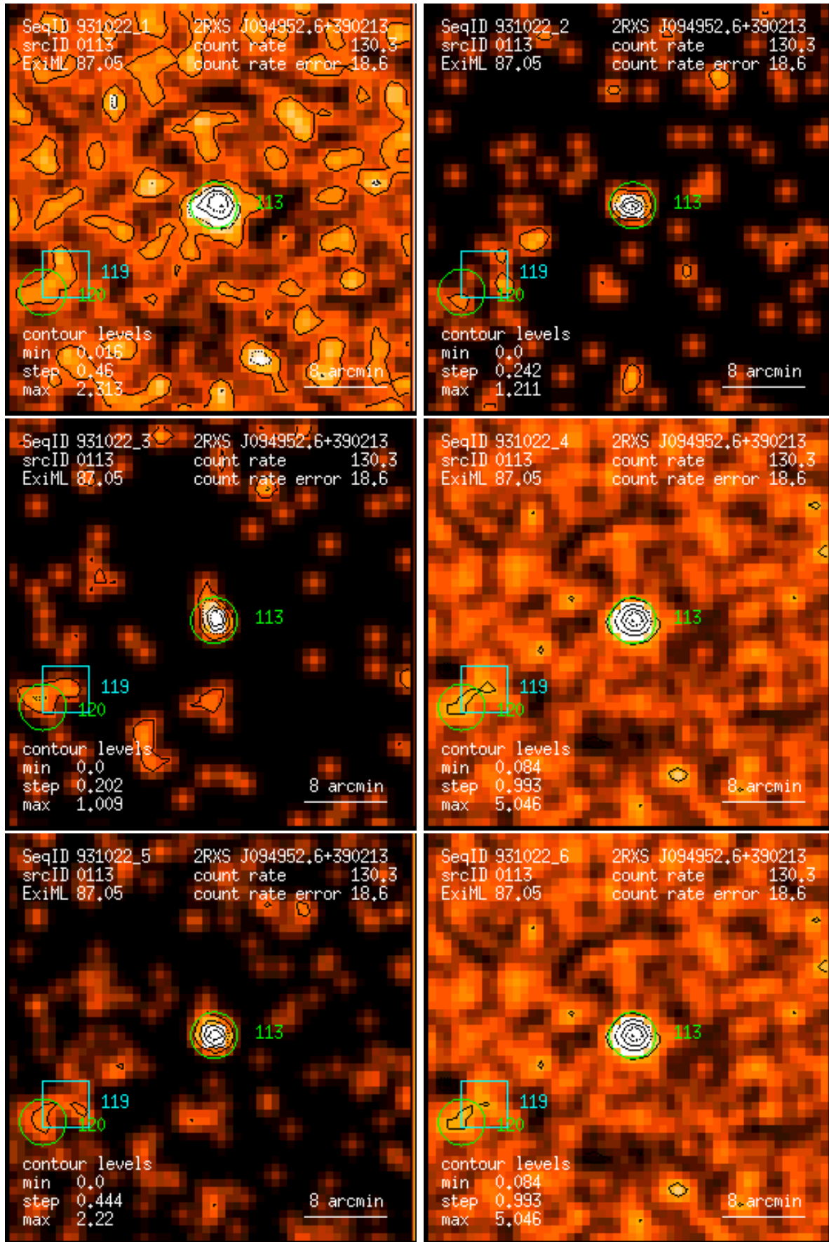
Figure 113: RASS 931022: detection 0113: band rate images, Gaussian filter: (1) PSPC channels 11 – 41, (2) 52 – 90, (3) 91 – 201, (4) 11 – 235, (5) 52 – 201, (6) 11 – 201. Broad band rates in counts/ks. Band rate contour levels in counts/ks/arcmin 2 .
