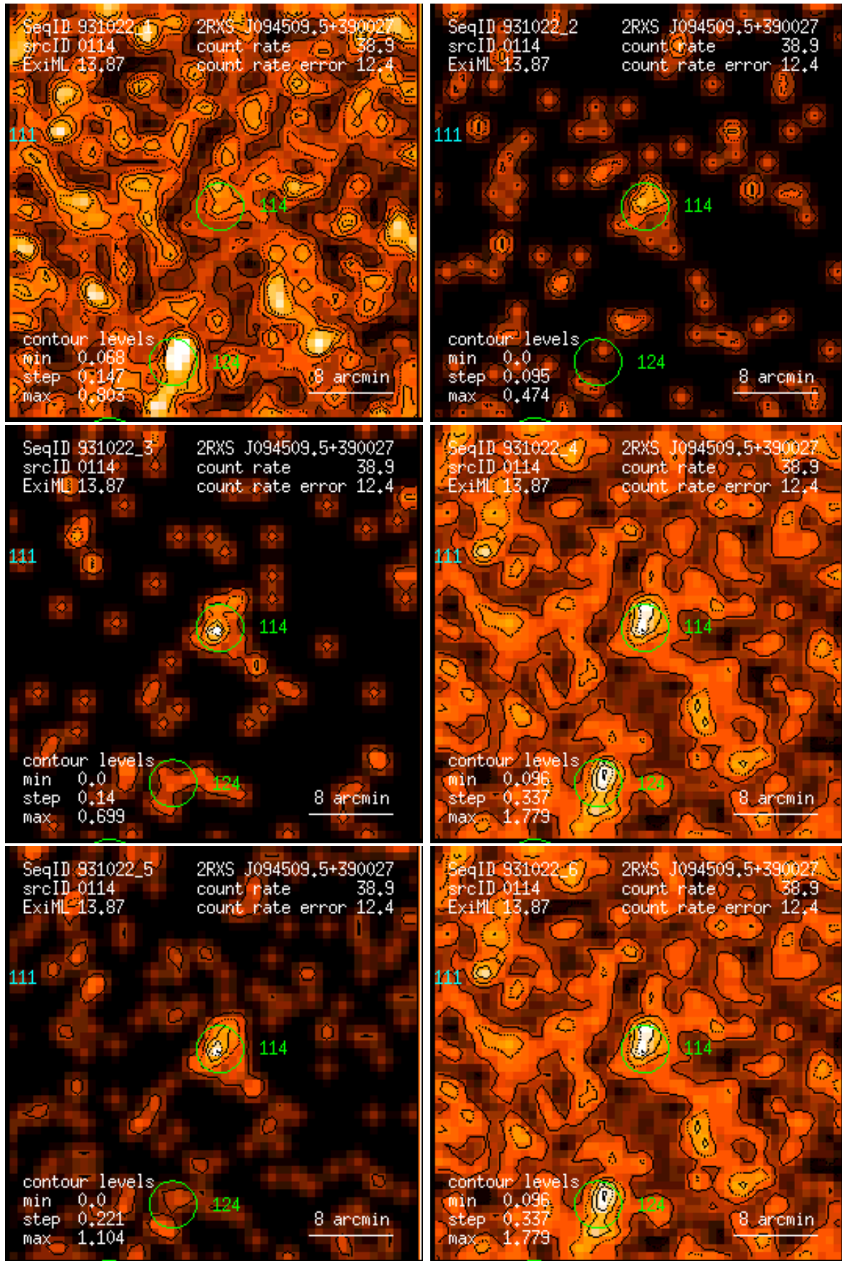
Figure 114: RASS 931022: detection 0114: band rate images, Gaussian filter: (1) PSPC channels 11 – 41, (2) 52 – 90, (3) 91 – 201, (4) 11 – 235, (5) 52 – 201, (6) 11 – 201. Broad band rates in counts/ks. Band rate contour levels in counts/ks/arcmin 2 .
