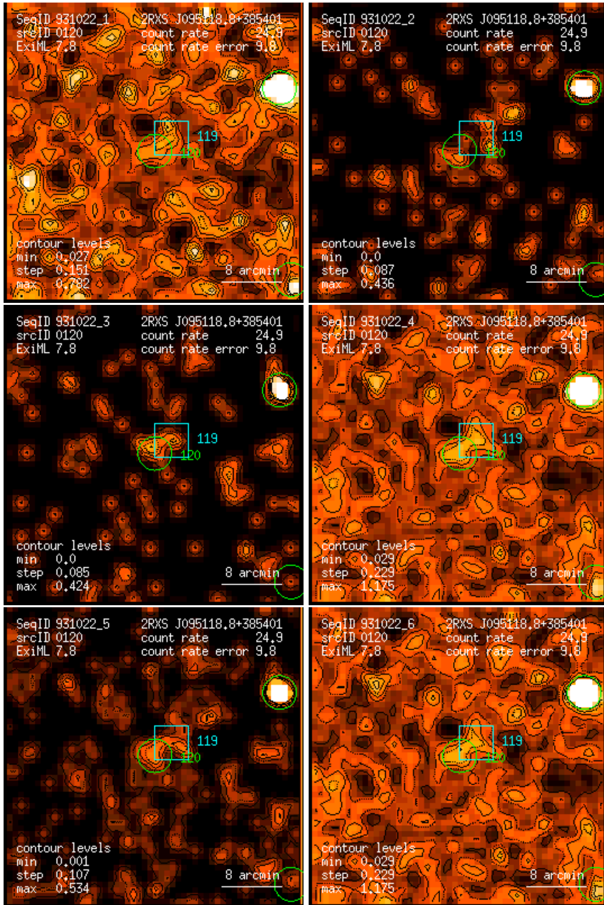
Figure 120: RASS 931022: detection 0120: band rate images, Gaussian filter: (1) PSPC channels 11 – 41, (2) 52 – 90, (3) 91 – 201, (4) 11 – 235, (5) 52 – 201, (6) 11 – 201. Broad band rates in counts/ks. Band rate contour levels in counts/ks/arcmin 2 .
