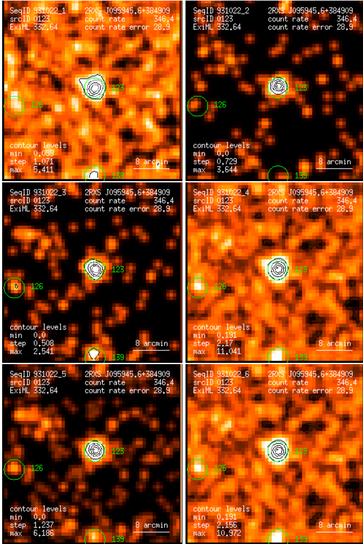
Figure 123: RASS 931022: detection 0123: band rate images, Gaussian filter: (1) PSPC channels 11 – 41, (2) 52 – 90, (3) 91 – 201, (4) 11 – 235, (5) 52 – 201, (6) 11 – 201. Broad band rates in counts/ks. Band rate contour levels in counts/ks/arcmin 2 .
