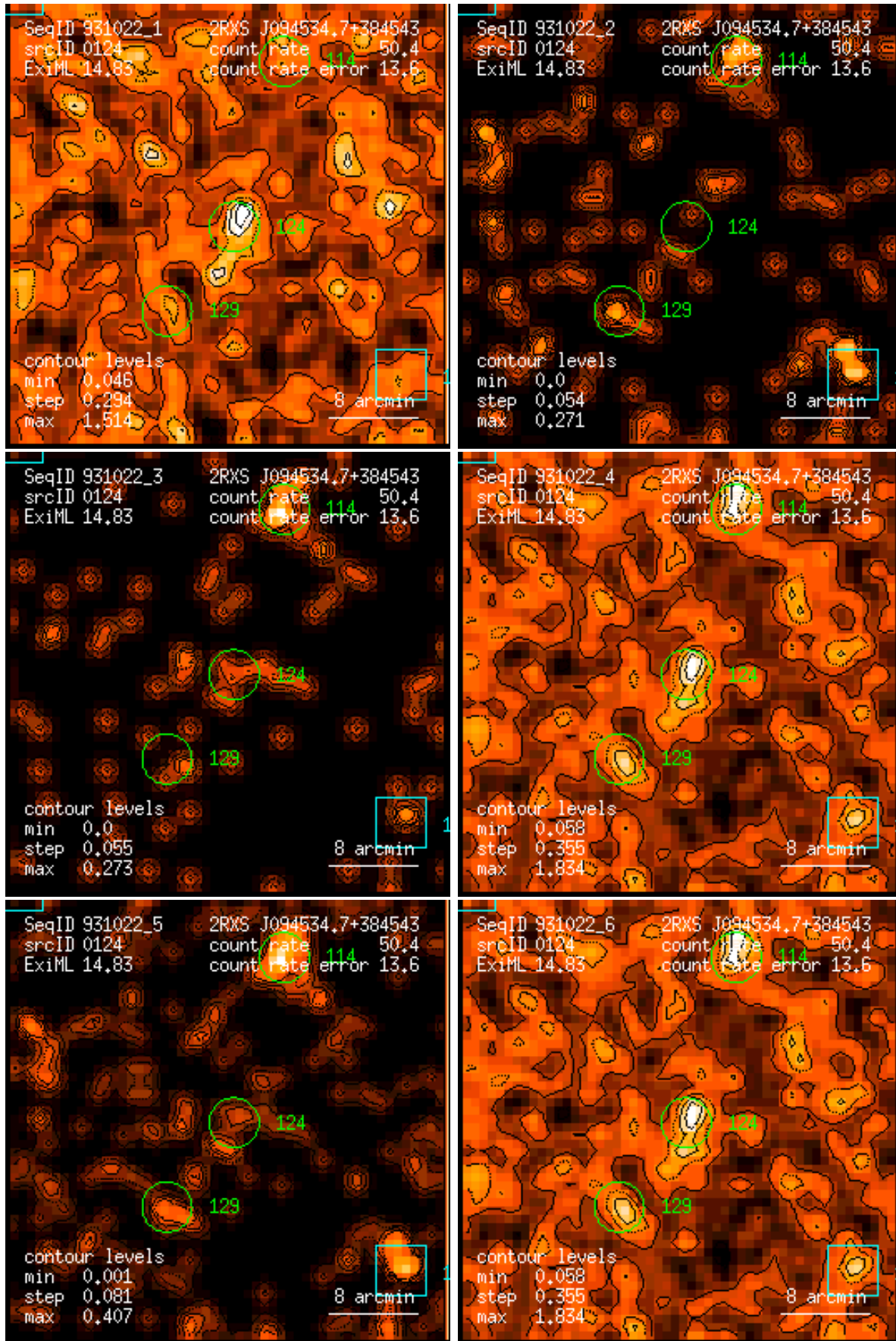
Figure 124: RASS 931022: detection 0124: band rate images, Gaussian filter: (1) PSPC channels 11 – 41, (2) 52 – 90, (3) 91 – 201, (4) 11 – 235, (5) 52 – 201, (6) 11 – 201. Broad band rates in counts/ks. Band rate contour levels in counts/ks/arcmin 2 .
