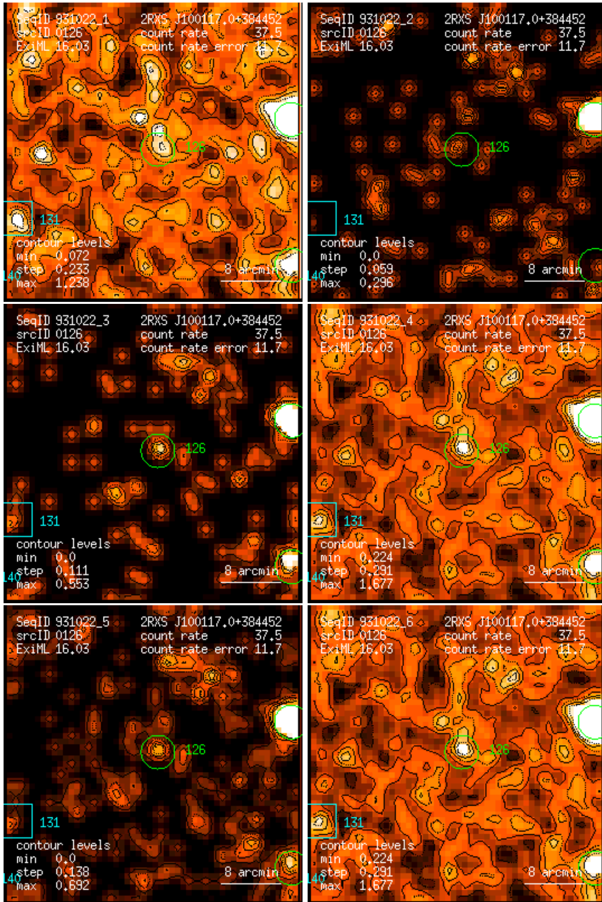
Figure 126: RASS 931022: detection 0126: band rate images, Gaussian filter: (1) PSPC channels 11 – 41, (2) 52 – 90, (3) 91 – 201, (4) 11 – 235, (5) 52 – 201, (6) 11 – 201. Broad band rates in counts/ks. Band rate contour levels in counts/ks/arcmin 2 .
