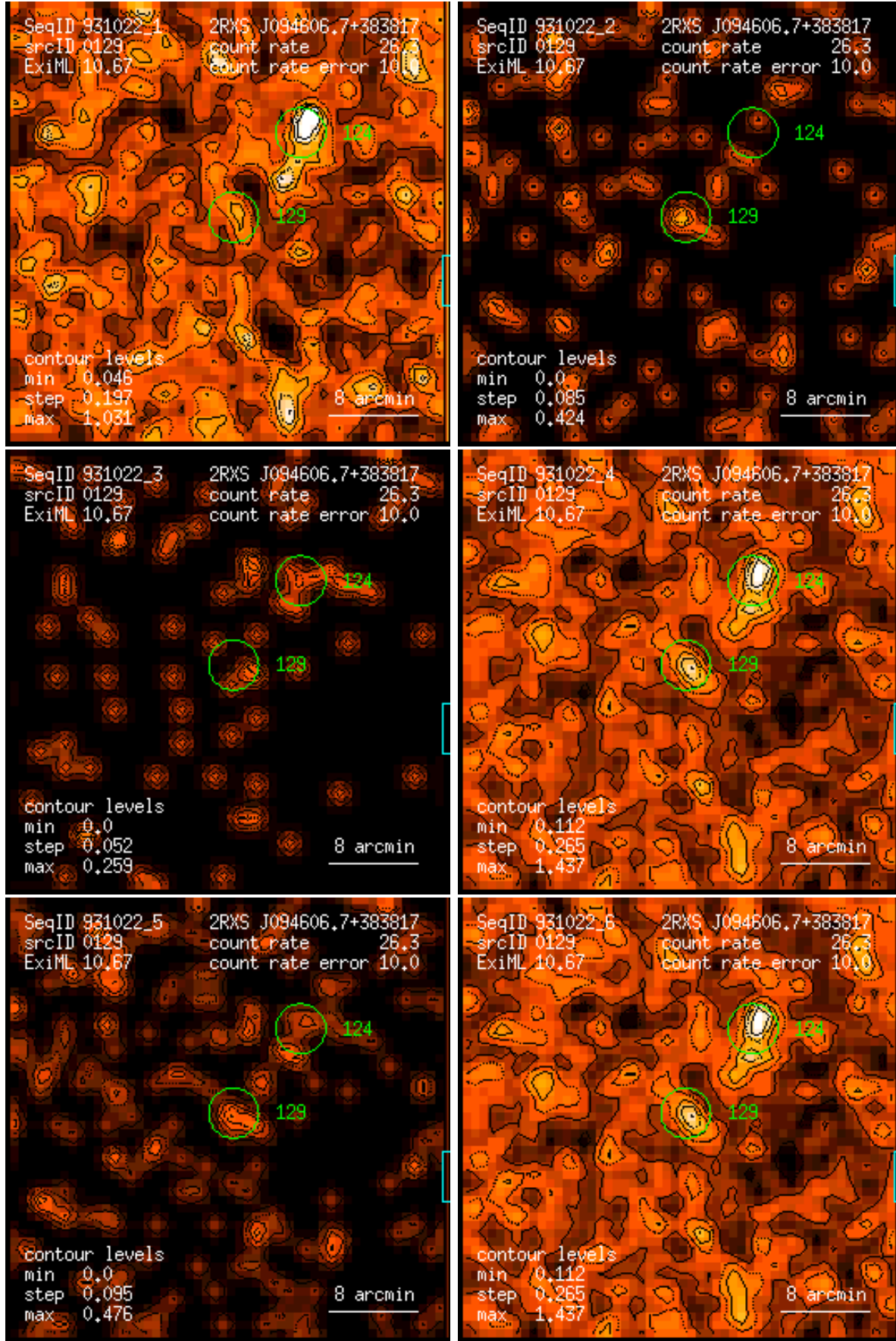
Figure 129: RASS 931022: detection 0129: band rate images, Gaussian filter: (1) PSPC channels 11 – 41, (2) 52 – 90, (3) 91 – 201, (4) 11 – 235, (5) 52 – 201, (6) 11 – 201. Broad band rates in counts/ks. Band rate contour levels in counts/ks/arcmin 2 .
