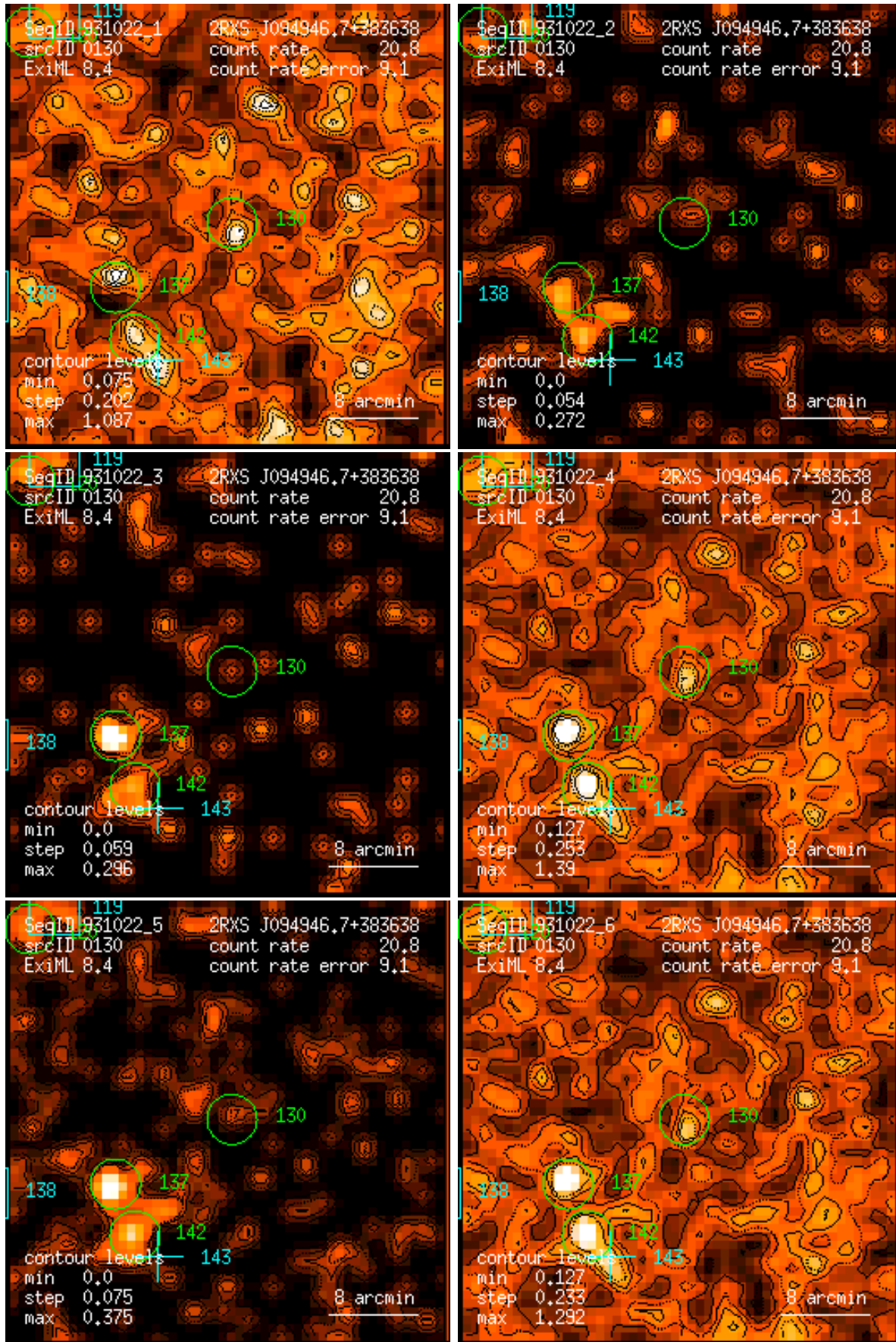
Figure 130: RASS 931022: detection 0130: band rate images, Gaussian filter: (1) PSPC channels 11 – 41, (2) 52 – 90, (3) 91 – 201, (4) 11 – 235, (5) 52 – 201, (6) 11 – 201. Broad band rates in counts/ks. Band rate contour levels in counts/ks/arcmin 2 .
