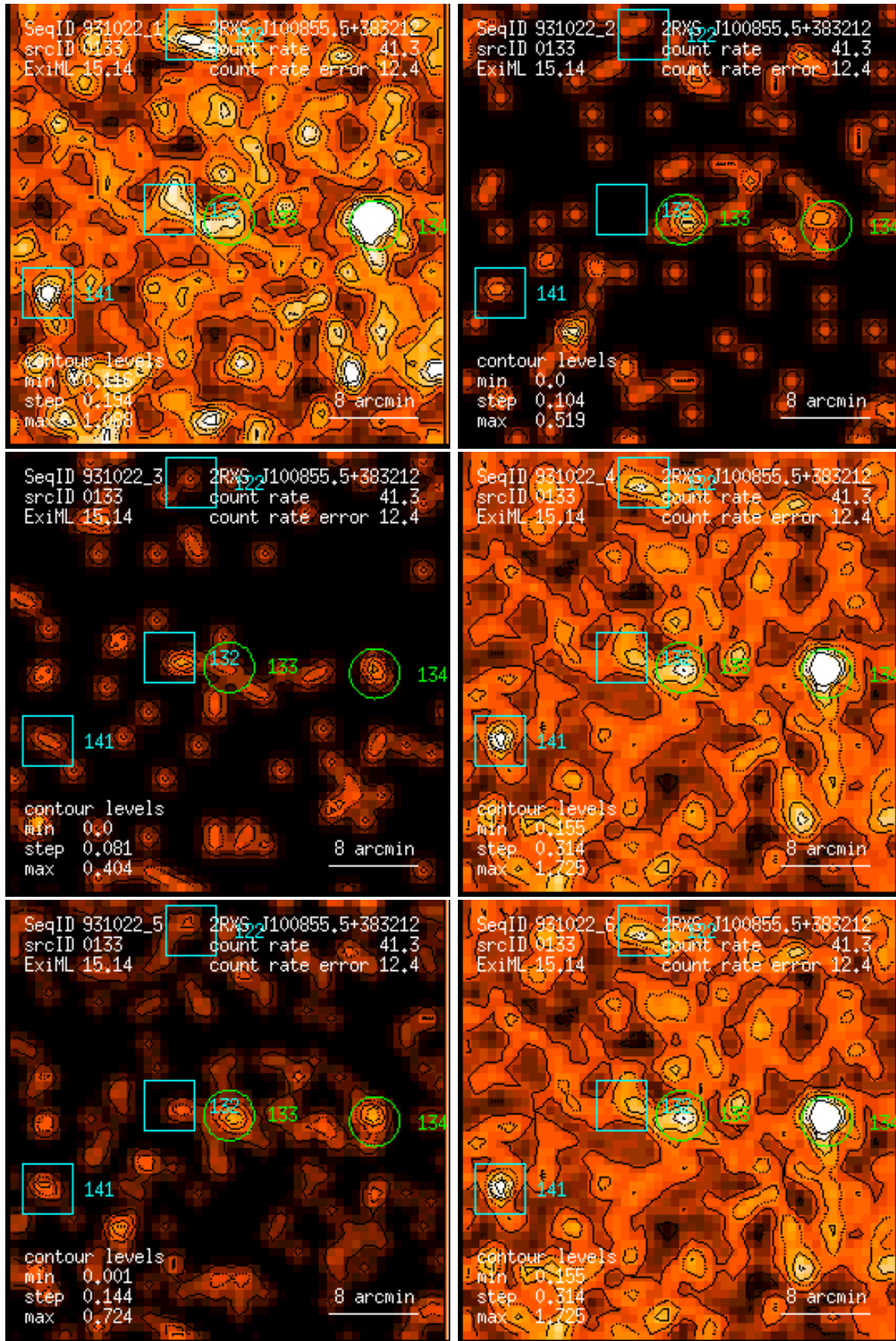
Figure 133: RASS 931022: detection 0133: band rate images, Gaussian filter: (1) PSPC channels 11 – 41, (2) 52 – 90, (3) 91 – 201, (4) 11 – 235, (5) 52 – 201, (6) 11 – 201. Broad band rates in counts/ks. Band rate contour levels in counts/ks/arcmin 2 .
