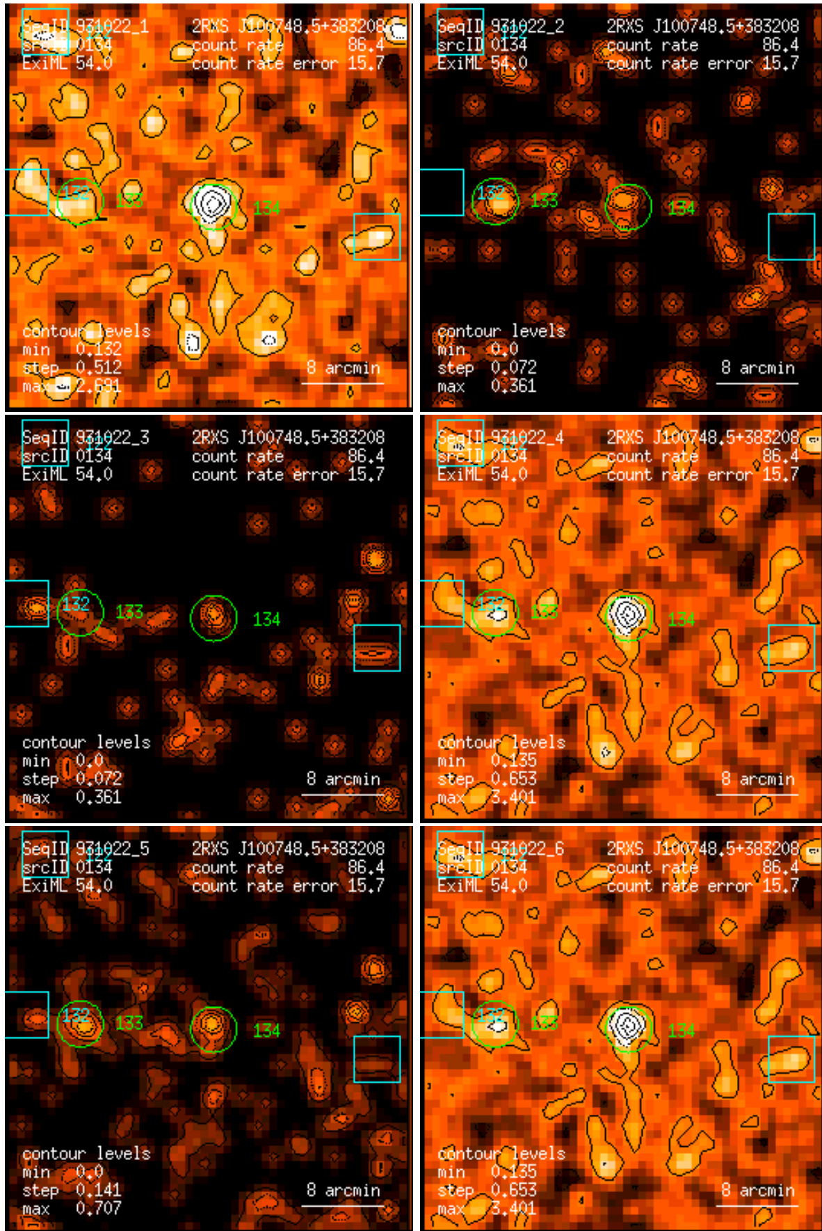
Figure 134: RASS 931022: detection 0134: band rate images, Gaussian filter: (1) PSPC channels 11 – 41, (2) 52 – 90, (3) 91 – 201, (4) 11 – 235, (5) 52 – 201, (6) 11 – 201. Broad band rates in counts/ks. Band rate contour levels in counts/ks/arcmin 2 .
