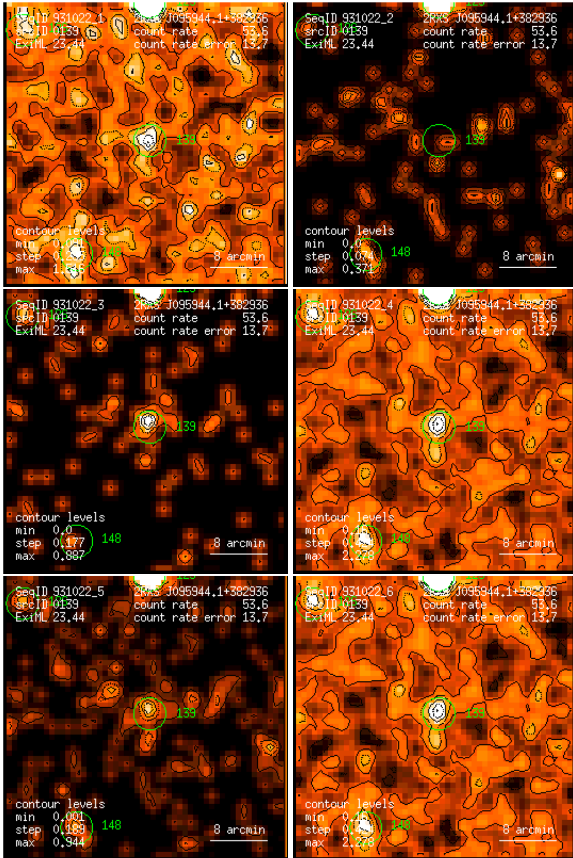
Figure 139: RASS 931022: detection 0139: band rate images, Gaussian filter: (1) PSPC channels 11 – 41, (2) 52 – 90, (3) 91 – 201, (4) 11 – 235, (5) 52 – 201, (6) 11 – 201. Broad band rates in counts/ks. Band rate contour levels in counts/ks/arcmin 2 .
