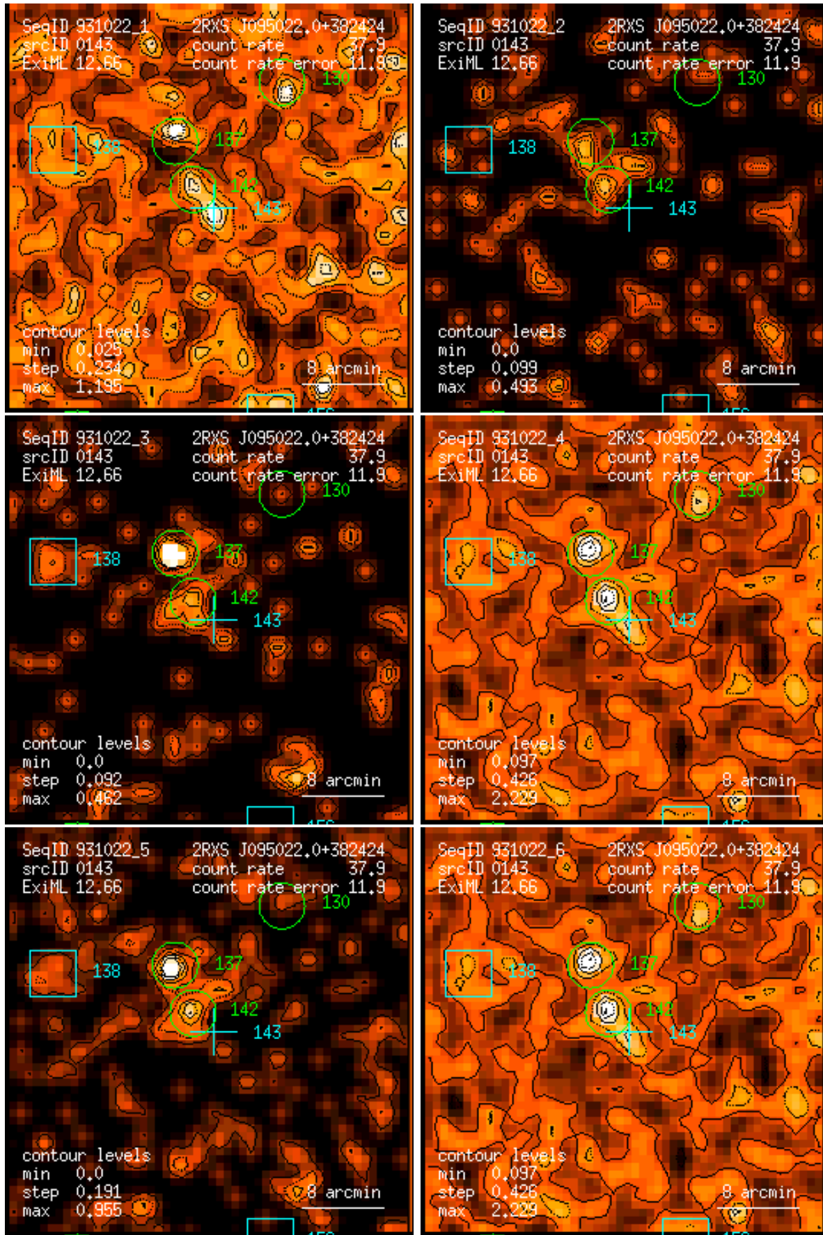
Figure 143: RASS 931022: detection 0143: band rate images, Gaussian filter: (1) PSPC channels 11 – 41, (2) 52 – 90, (3) 91 – 201, (4) 11 – 235, (5) 52 – 201, (6) 11 – 201. Broad band rates in counts/ks. Band rate contour levels in counts/ks/arcmin 2 .
