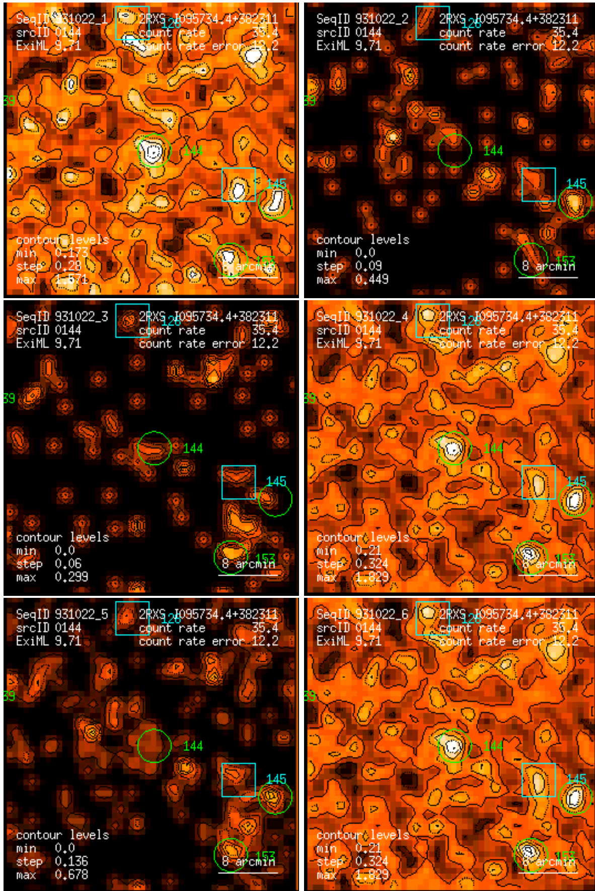
Figure 144: RASS 931022: detection 0144: band rate images, Gaussian filter: (1) PSPC channels 11 – 41, (2) 52 – 90, (3) 91 – 201, (4) 11 – 235, (5) 52 – 201, (6) 11 – 201. Broad band rates in counts/ks. Band rate contour levels in counts/ks/arcmin 2 .
