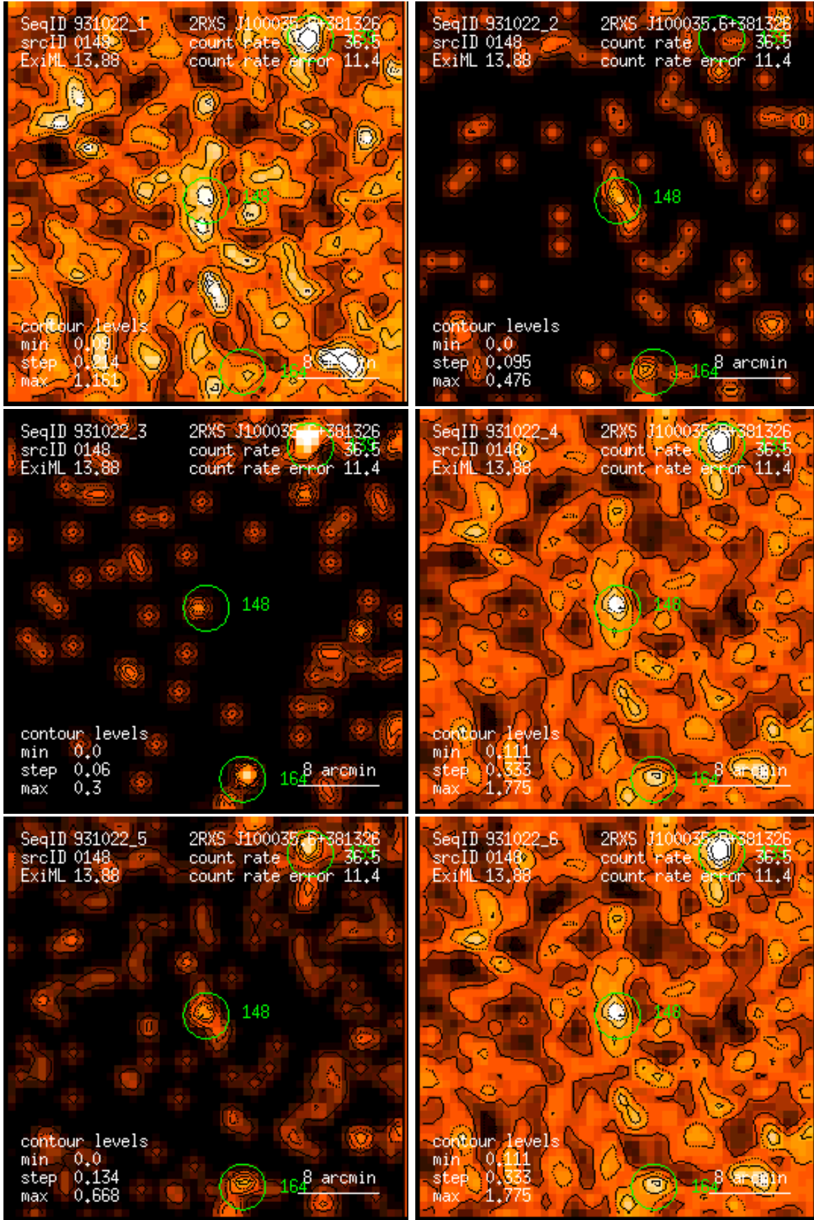
Figure 148: RASS 931022: detection 0148: band rate images, Gaussian filter: (1) PSPC channels 11 – 41, (2) 52 – 90, (3) 91 – 201, (4) 11 – 235, (5) 52 – 201, (6) 11 – 201. Broad band rates in counts/ks. Band rate contour levels in counts/ks/arcmin 2 .
