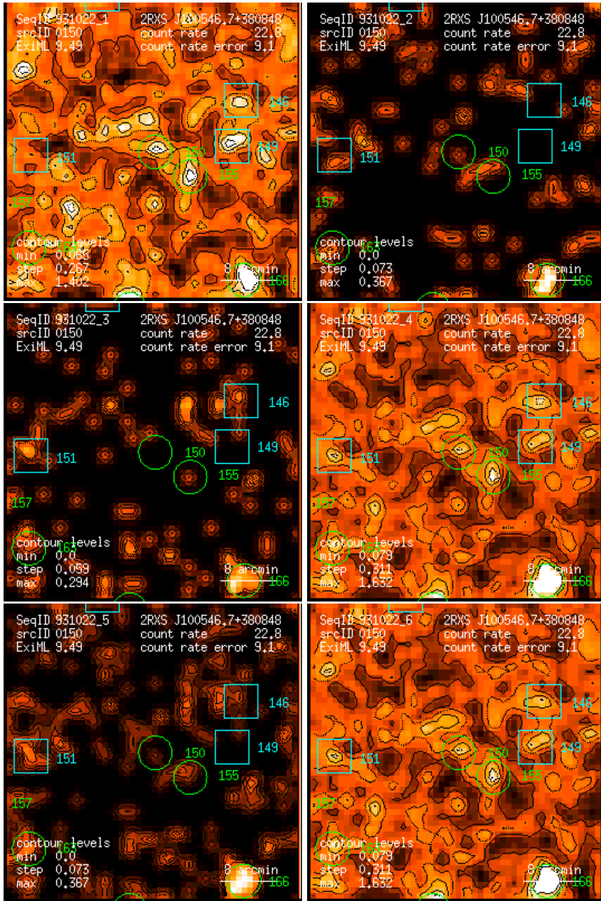
Figure 150: RASS 931022: detection 0150: band rate images, Gaussian filter: (1) PSPC channels 11 – 41, (2) 52 – 90, (3) 91 – 201, (4) 11 – 235, (5) 52 – 201, (6) 11 – 201. Broad band rates in counts/ks. Band rate contour levels in counts/ks/arcmin 2 .
