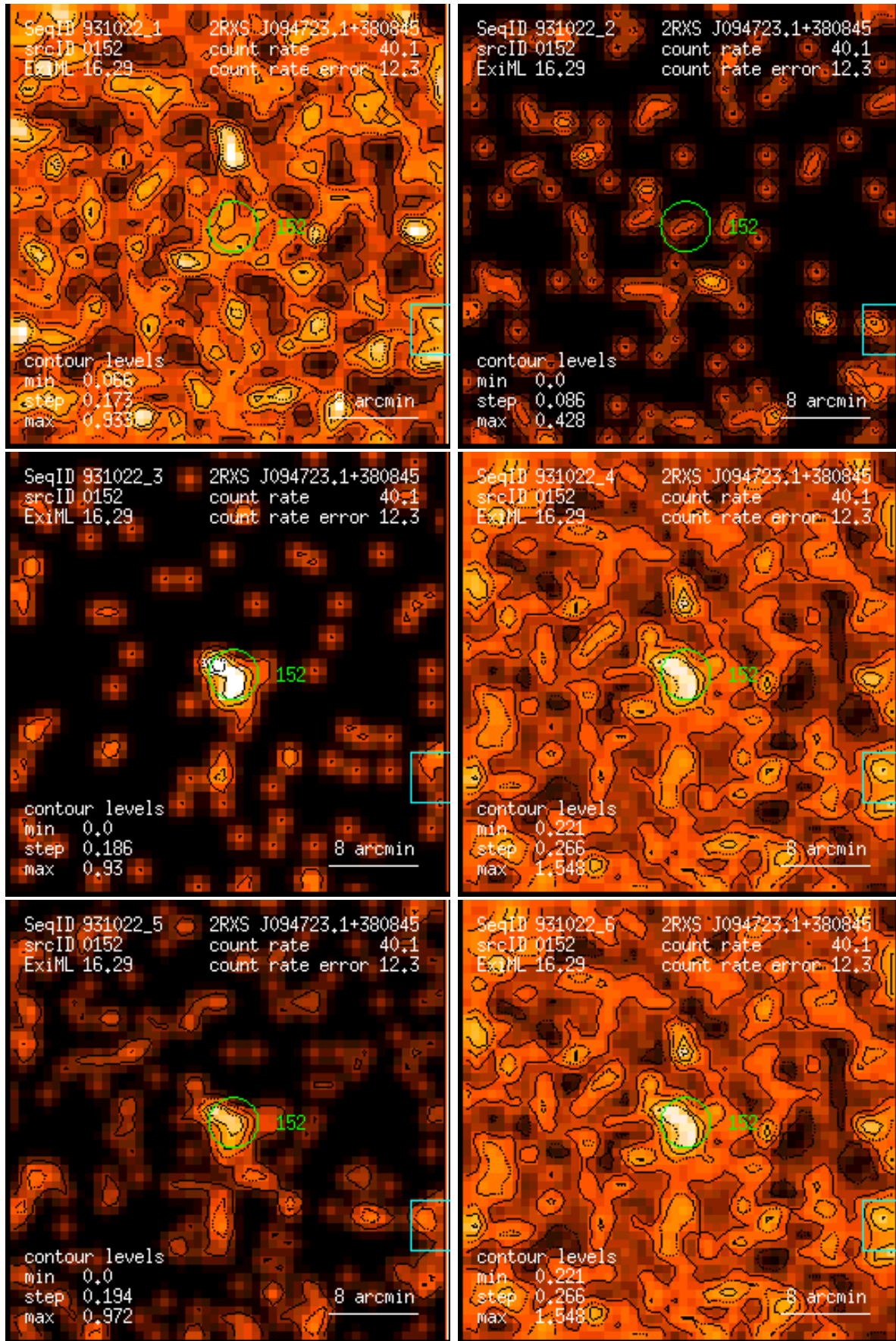
Figure 152: RASS 931022: detection 0152: band rate images, Gaussian filter: (1) PSPC channels 11 – 41, (2) 52 – 90, (3) 91 – 201, (4) 11 – 235, (5) 52 – 201, (6) 11 – 201. Broad band rates in counts/ks. Band rate contour levels in counts/ks/arcmin 2 .
