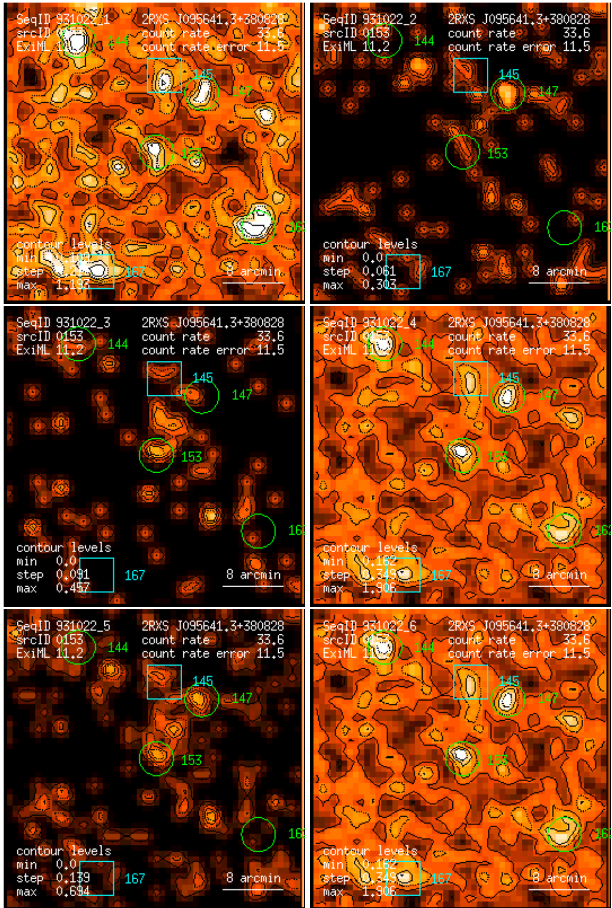
Figure 153: RASS 931022: detection 0153: band rate images, Gaussian filter: (1) PSPC channels 11 – 41, (2) 52 – 90, (3) 91 – 201, (4) 11 – 235, (5) 52 – 201, (6) 11 – 201. Broad band rates in counts/ks. Band rate contour levels in counts/ks/arcmin 2 .
