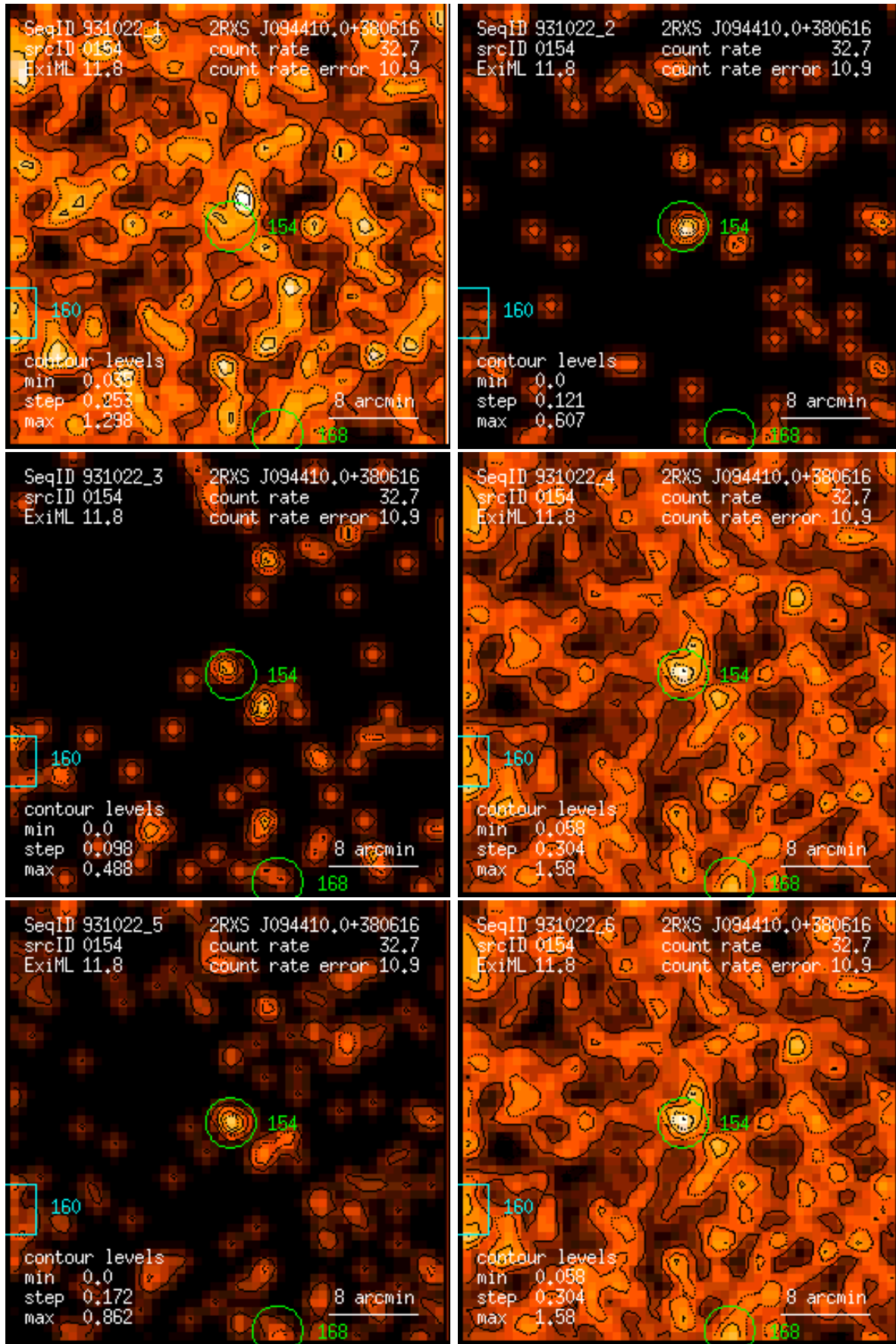
Figure 154: RASS 931022: detection 0154: band rate images, Gaussian filter: (1) PSPC channels 11 – 41, (2) 52 – 90, (3) 91 – 201, (4) 11 – 235, (5) 52 – 201, (6) 11 – 201. Broad band rates in counts/ks. Band rate contour levels in counts/ks/arcmin 2 .
