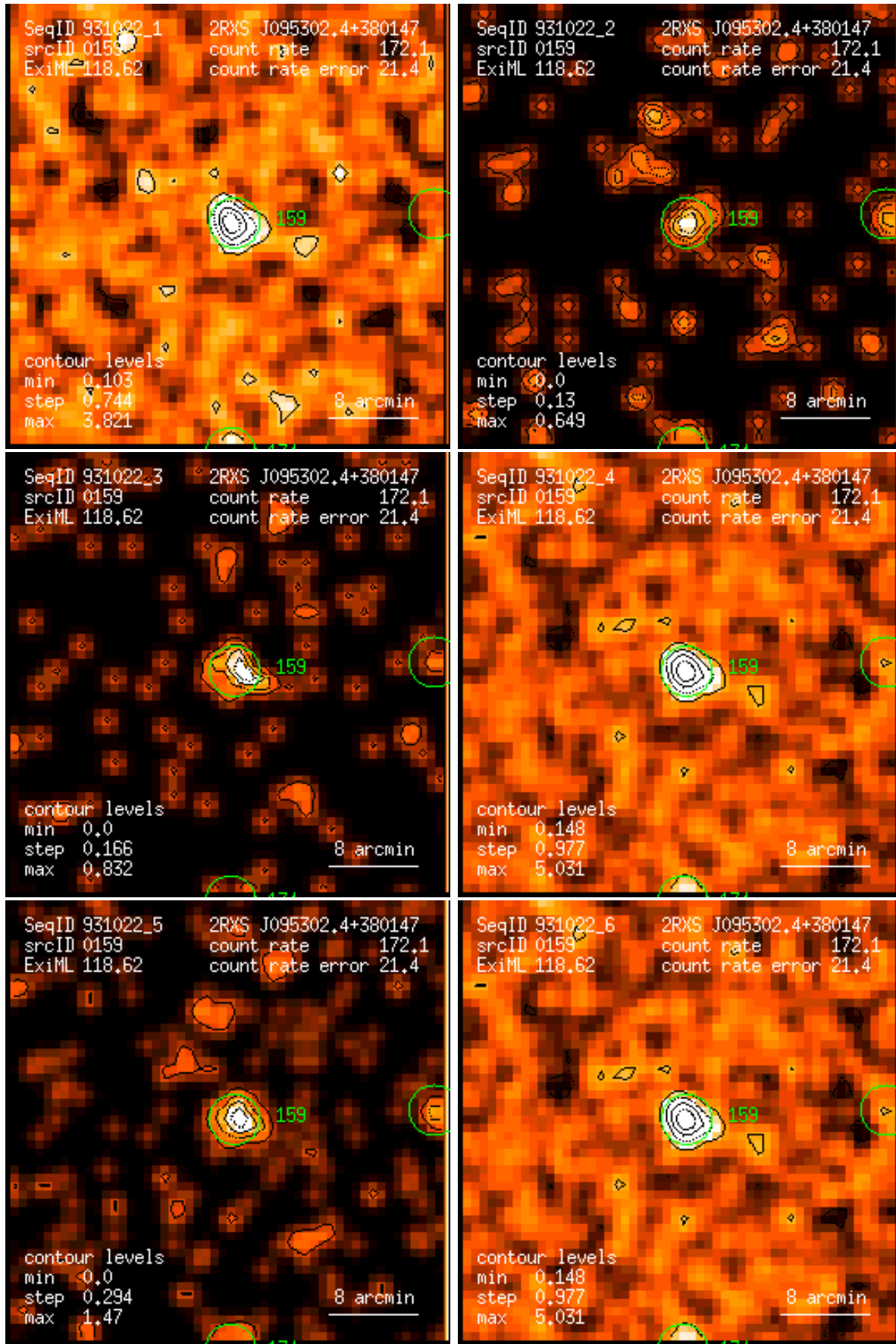
Figure 159: RASS 931022: detection 0159: band rate images, Gaussian filter: (1) PSPC channels 11 – 41, (2) 52 – 90, (3) 91 – 201, (4) 11 – 235, (5) 52 – 201, (6) 11 – 201. Broad band rates in counts/ks. Band rate contour levels in counts/ks/arcmin 2 .
