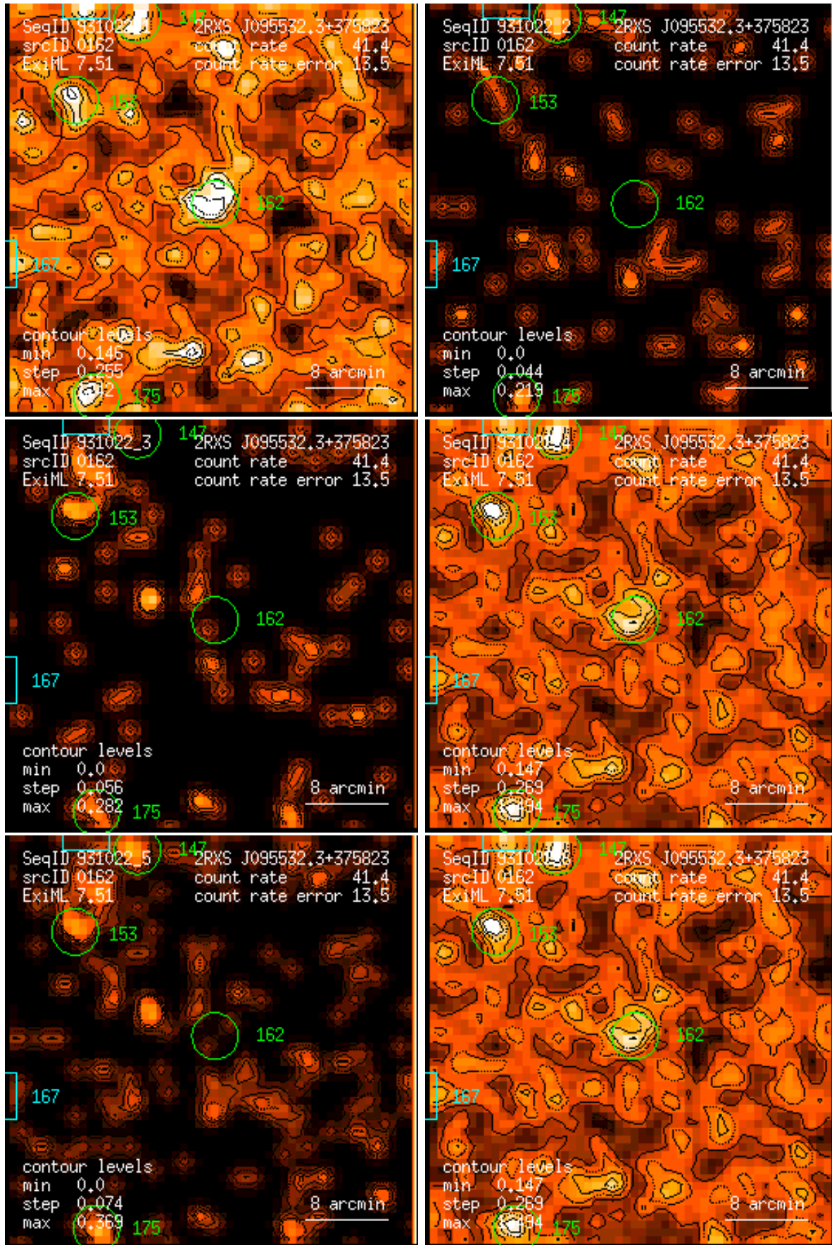
Figure 162: RASS 931022: detection 0162: band rate images, Gaussian filter: (1) PSPC channels 11 – 41, (2) 52 – 90, (3) 91 – 201, (4) 11 – 235, (5) 52 – 201, (6) 11 – 201. Broad band rates in counts/ks. Band rate contour levels in counts/ks/arcmin 2 .
