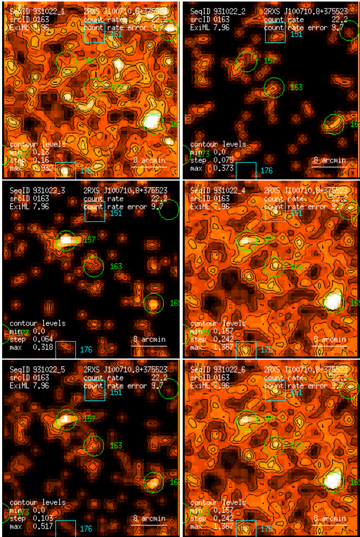
Figure 163: RASS 931022: detection 0163: band rate images, Gaussian filter: (1) PSPC channels 11 – 41, (2) 52 – 90, (3) 91 – 201, (4) 11 – 235, (5) 52 – 201, (6) 11 – 201. Broad band rates in counts/ks. Band rate contour levels in counts/ks/arcmin 2 .
