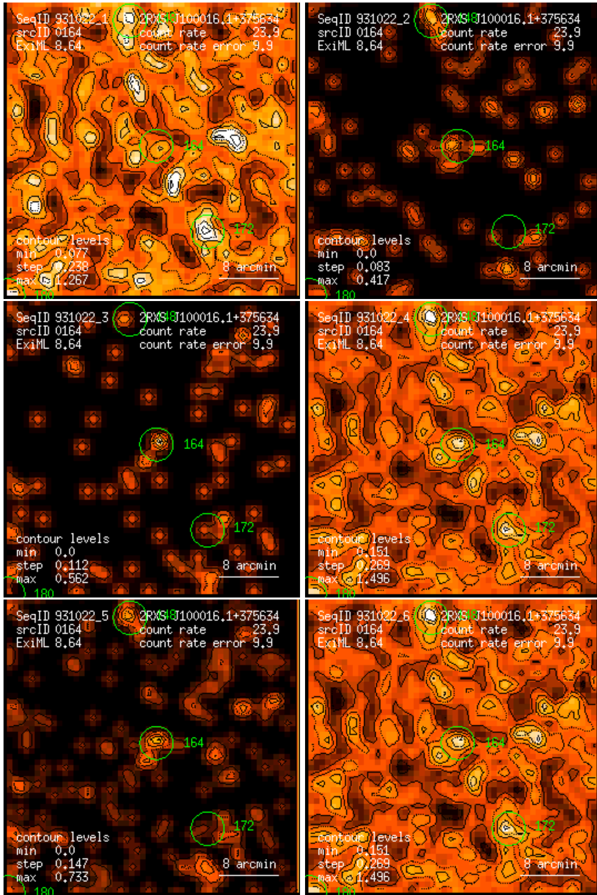
Figure 164: RASS 931022: detection 0164: band rate images, Gaussian filter: (1) PSPC channels 11 – 41, (2) 52 – 90, (3) 91 – 201, (4) 11 – 235, (5) 52 – 201, (6) 11 – 201. Broad band rates in counts/ks. Band rate contour levels in counts/ks/arcmin 2 .
