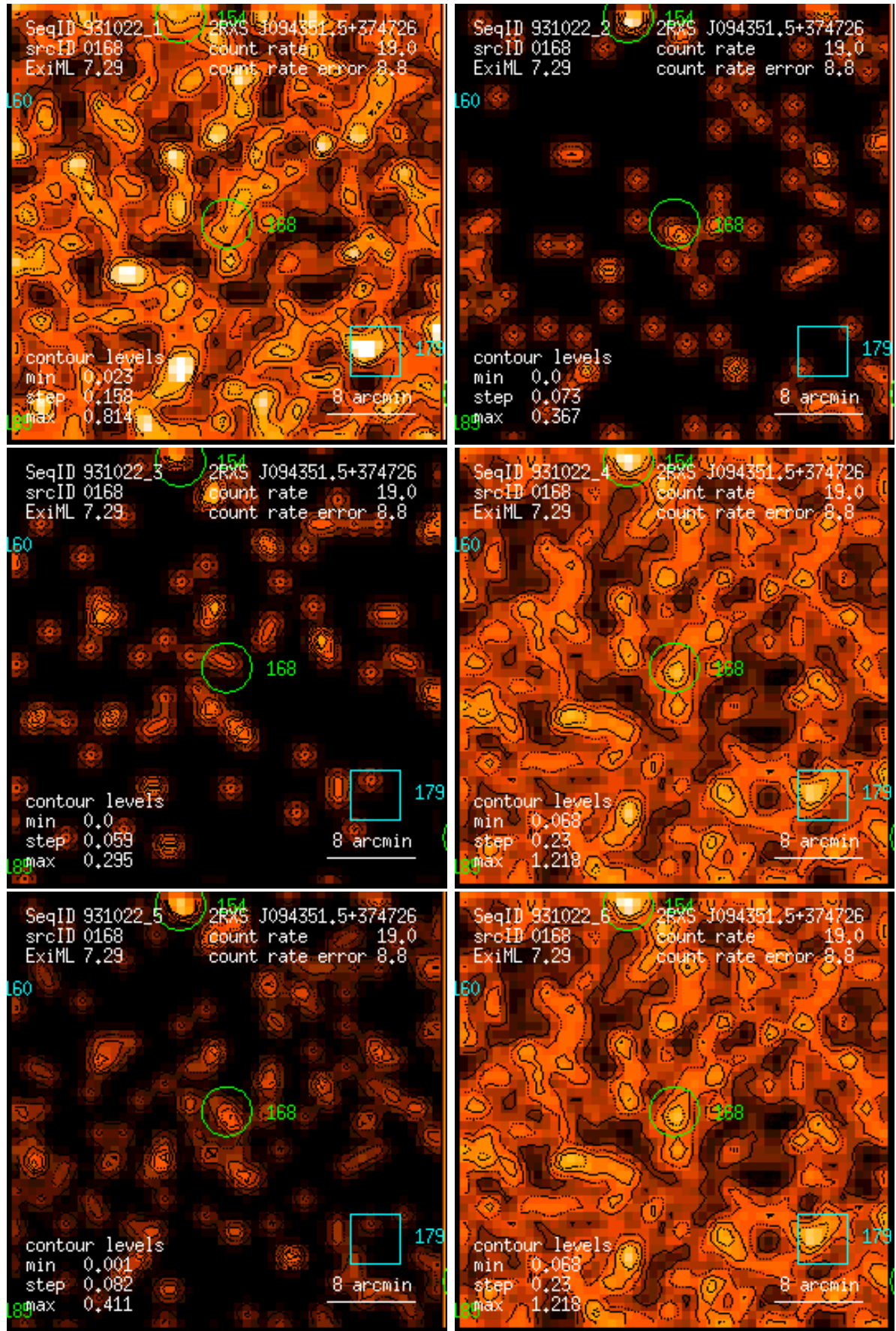
Figure 168: RASS 931022: detection 0168: band rate images, Gaussian filter: (1) PSPC channels 11 – 41, (2) 52 – 90, (3) 91 – 201, (4) 11 – 235, (5) 52 – 201, (6) 11 – 201. Broad band rates in counts/ks. Band rate contour levels in counts/ks/arcmin 2 .
