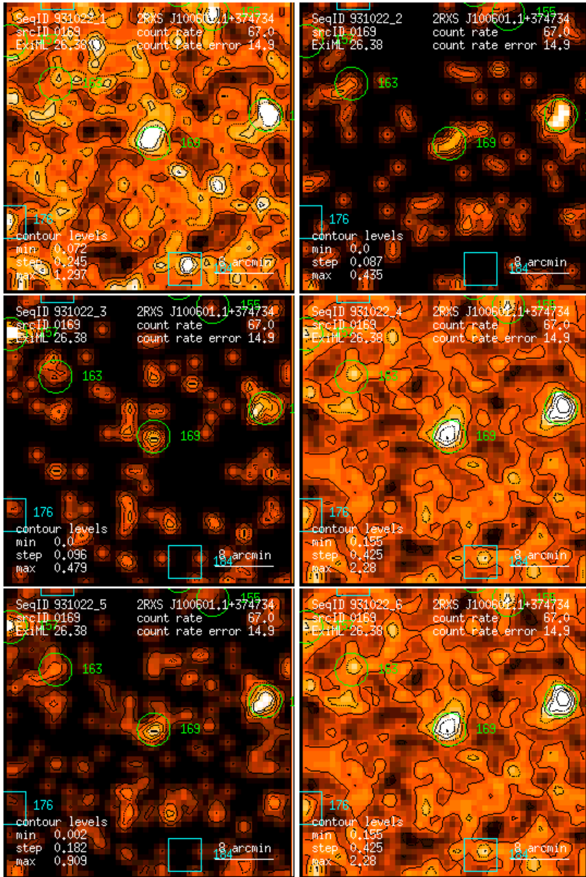
Figure 169: RASS 931022: detection 0169: band rate images, Gaussian filter: (1) PSPC channels 11 – 41, (2) 52 – 90, (3) 91 – 201, (4) 11 – 235, (5) 52 – 201, (6) 11 – 201. Broad band rates in counts/ks. Band rate contour levels in counts/ks/arcmin 2 .
