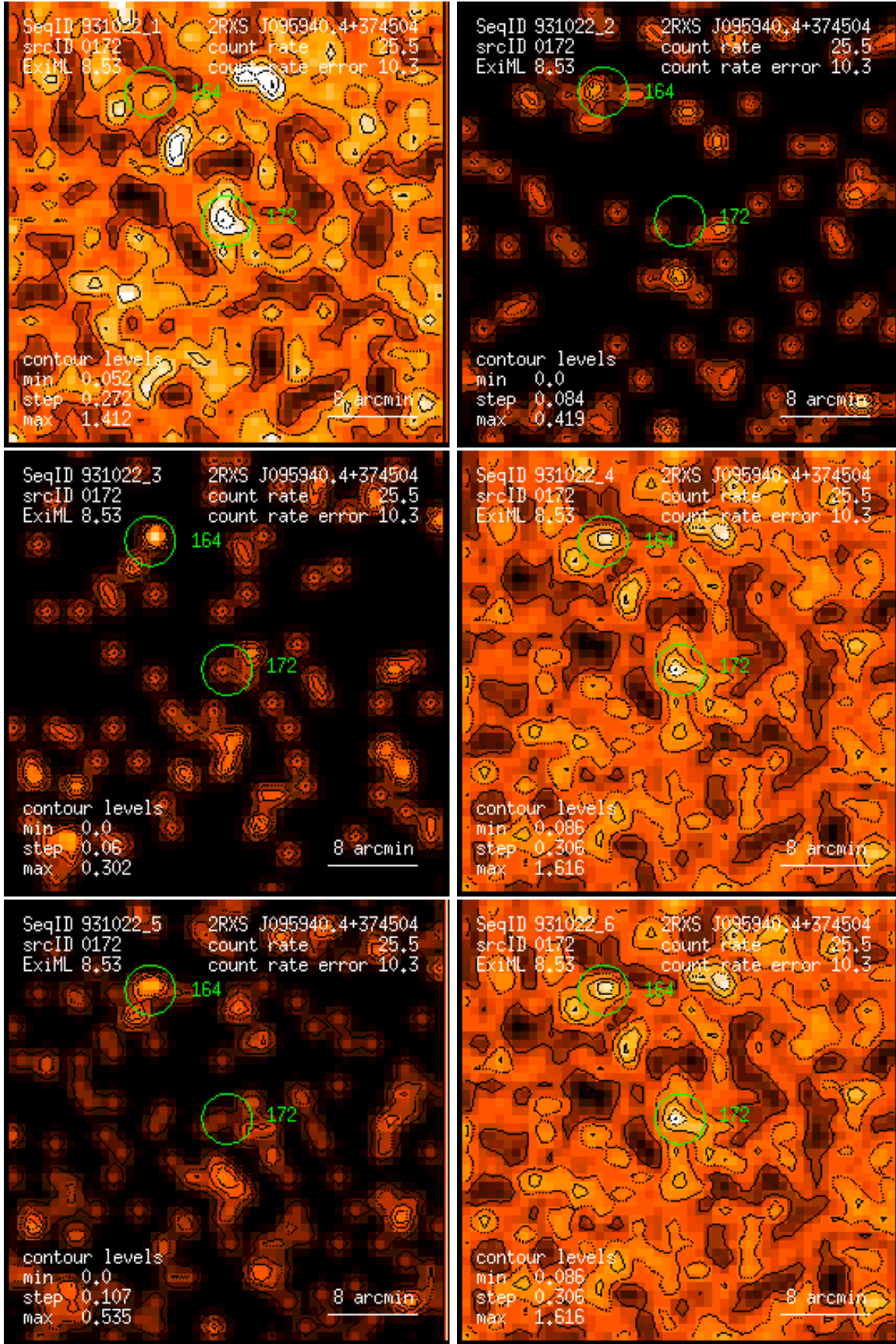
Figure 172: RASS 931022: detection 0172: band rate images, Gaussian filter: (1) PSPC channels 11 – 41, (2) 52 – 90, (3) 91 – 201, (4) 11 – 235, (5) 52 – 201, (6) 11 – 201. Broad band rates in counts/ks. Band rate contour levels in counts/ks/arcmin 2 .
