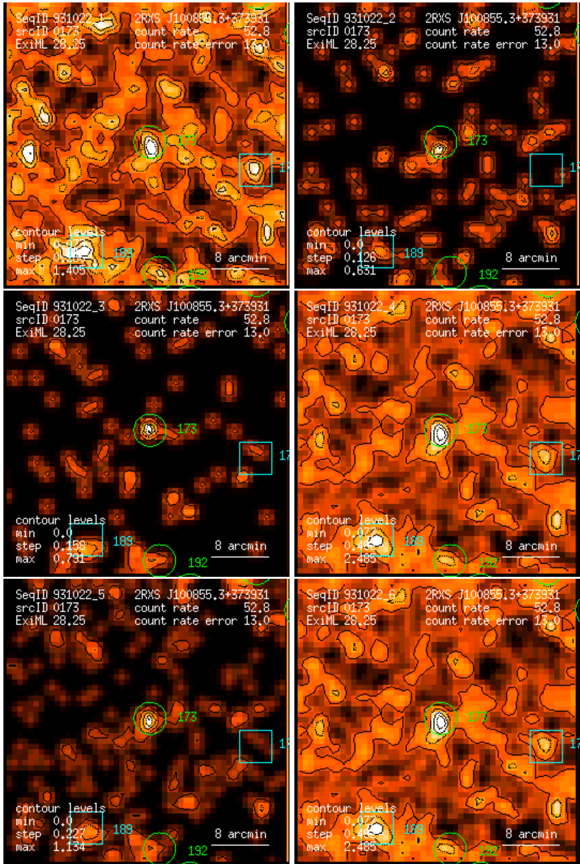
Figure 173: RASS 931022: detection 0173: band rate images, Gaussian filter: (1) PSPC channels 11 – 41, (2) 52 – 90, (3) 91 – 201, (4) 11 – 235, (5) 52 – 201, (6) 11 – 201. Broad band rates in counts/ks. Band rate contour levels in counts/ks/arcmin 2 .
