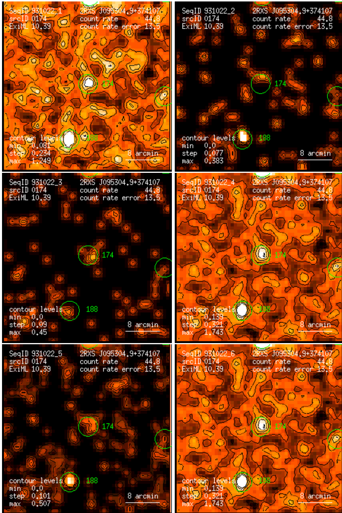
Figure 174: RASS 931022: detection 0174: band rate images, Gaussian filter: (1) PSPC channels 11 – 41, (2) 52 – 90, (3) 91 – 201, (4) 11 – 235, (5) 52 – 201, (6) 11 – 201. Broad band rates in counts/ks. Band rate contour levels in counts/ks/arcmin 2 .
