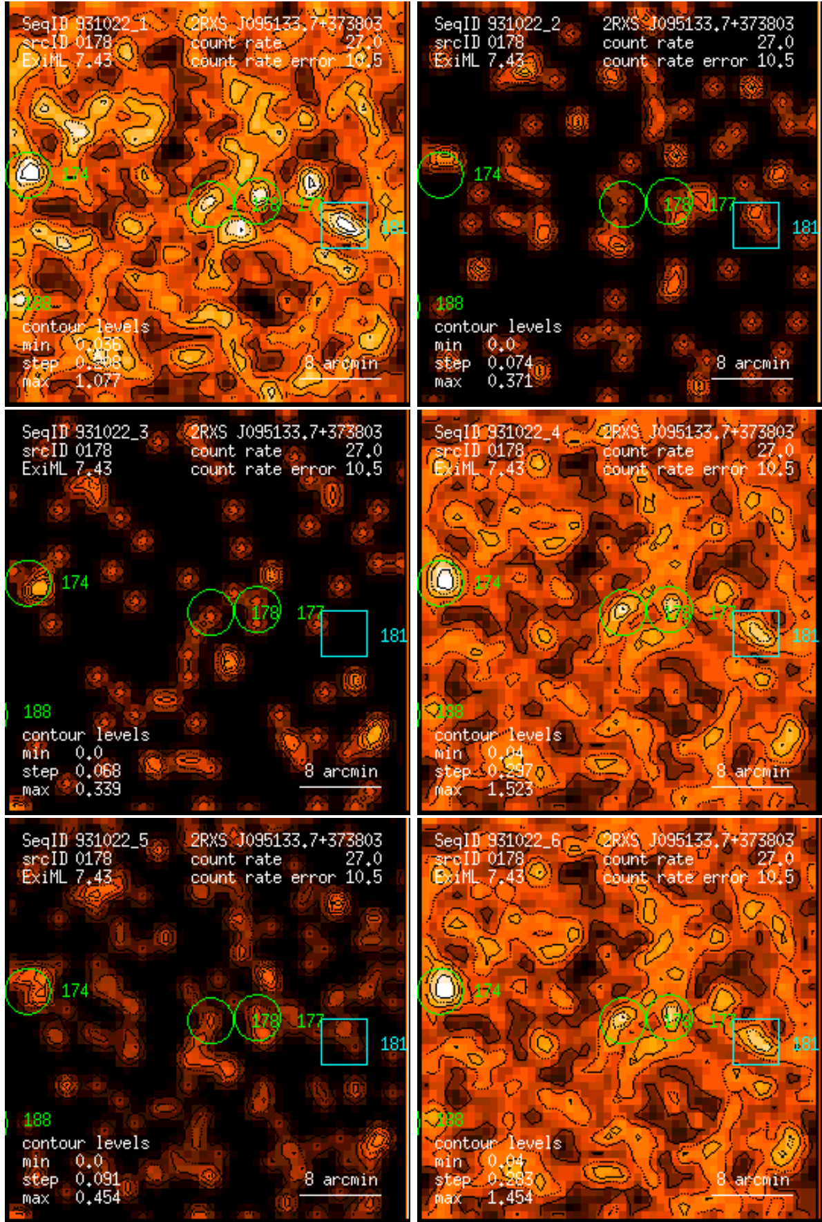
Figure 178: RASS 931022: detection 0178: band rate images, Gaussian filter: (1) PSPC channels 11 – 41, (2) 52 – 90, (3) 91 – 201, (4) 11 – 235, (5) 52 – 201, (6) 11 – 201. Broad band rates in counts/ks. Band rate contour levels in counts/ks/arcmin 2 .
